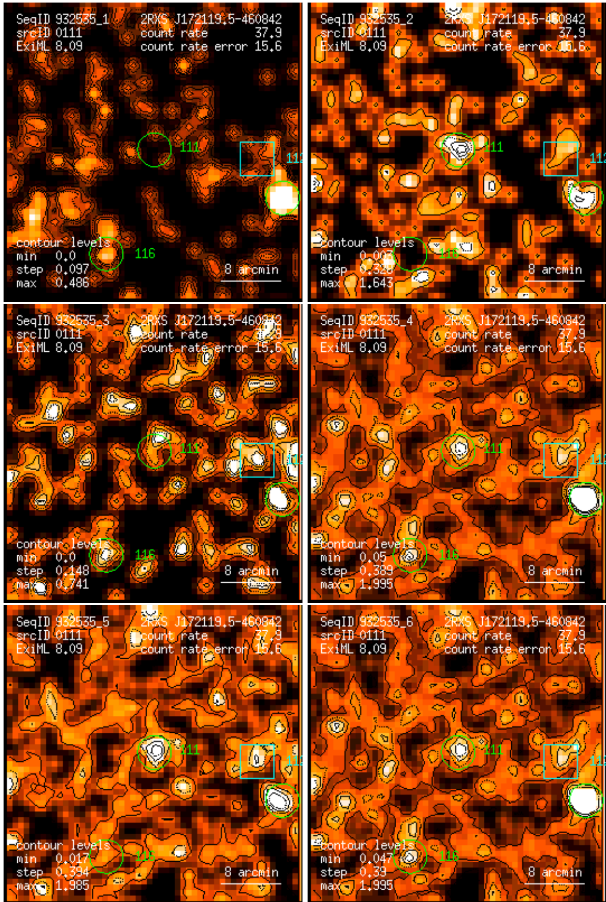
Figure 111: RASS 932535: detection 0111: band rate images, Gaussian filter: (1) PSPC channels 11 – 41, (2) 52 – 90, (3) 91 – 201, (4) 11 – 235, (5) 52 – 201, (6) 11 – 201. Broad band rates in counts/ks. Band rate contour levels in counts/ks/arcmin 2 .
