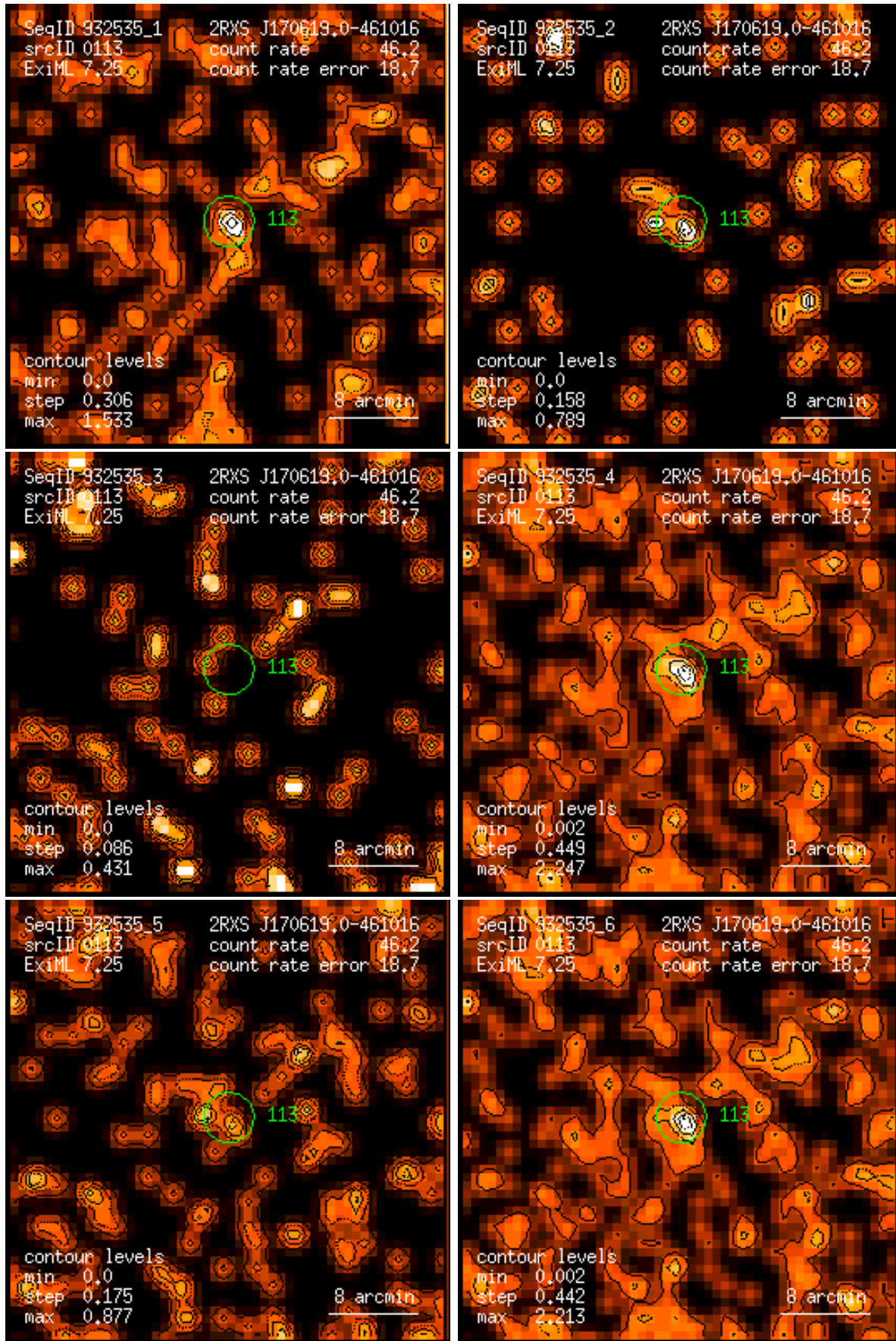
Figure 113: RASS 932535: detection 0113: band rate images, Gaussian filter: (1) PSPC channels 11 – 41, (2) 52 – 90, (3) 91 – 201, (4) 11 – 235, (5) 52 – 201, (6) 11 – 201. Broad band rates in counts/ks. Band rate contour levels in counts/ks/arcmin 2 .
