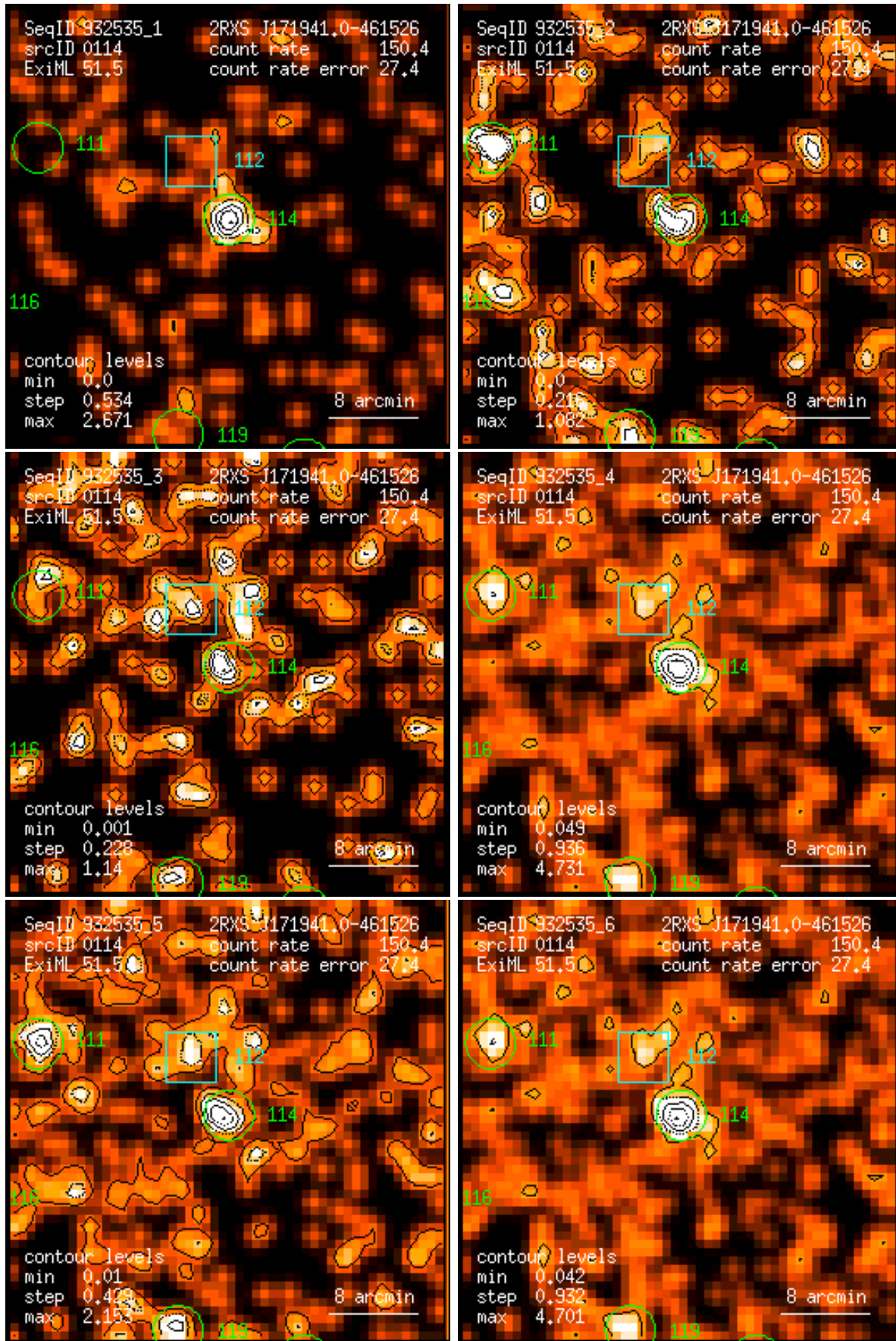
Figure 114: RASS 932535: detection 0114: band rate images, Gaussian filter: (1) PSPC channels 11 – 41, (2) 52 – 90, (3) 91 – 201, (4) 11 – 235, (5) 52 – 201, (6) 11 – 201. Broad band rates in counts/ks. Band rate contour levels in counts/ks/arcmin 2 .
