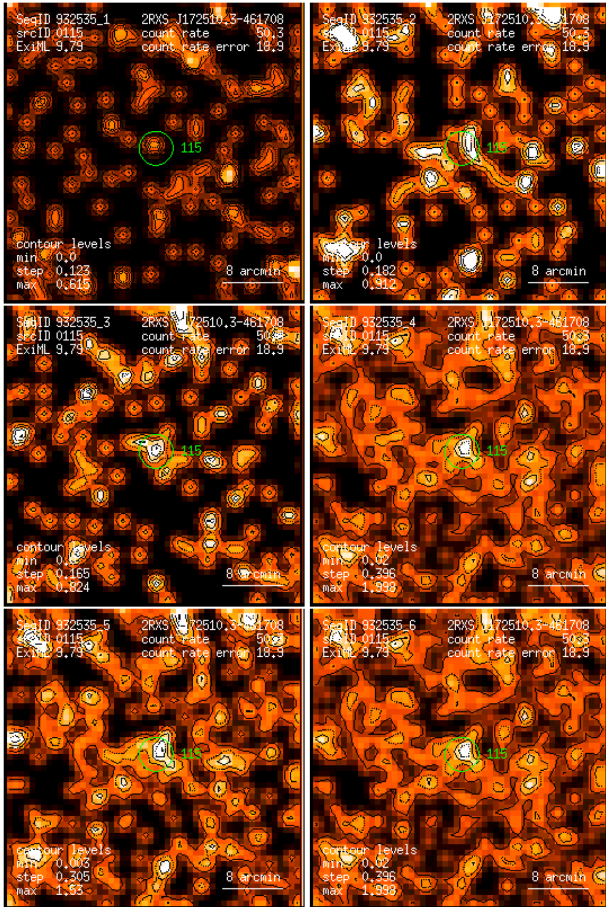
Figure 115: RASS 932535: detection 0115: band rate images, Gaussian filter: (1) PSPC channels 11 – 41, (2) 52 – 90, (3) 91 – 201, (4) 11 – 235, (5) 52 – 201, (6) 11 – 201. Broad band rates in counts/ks. Band rate contour levels in counts/ks/arcmin 2 .
