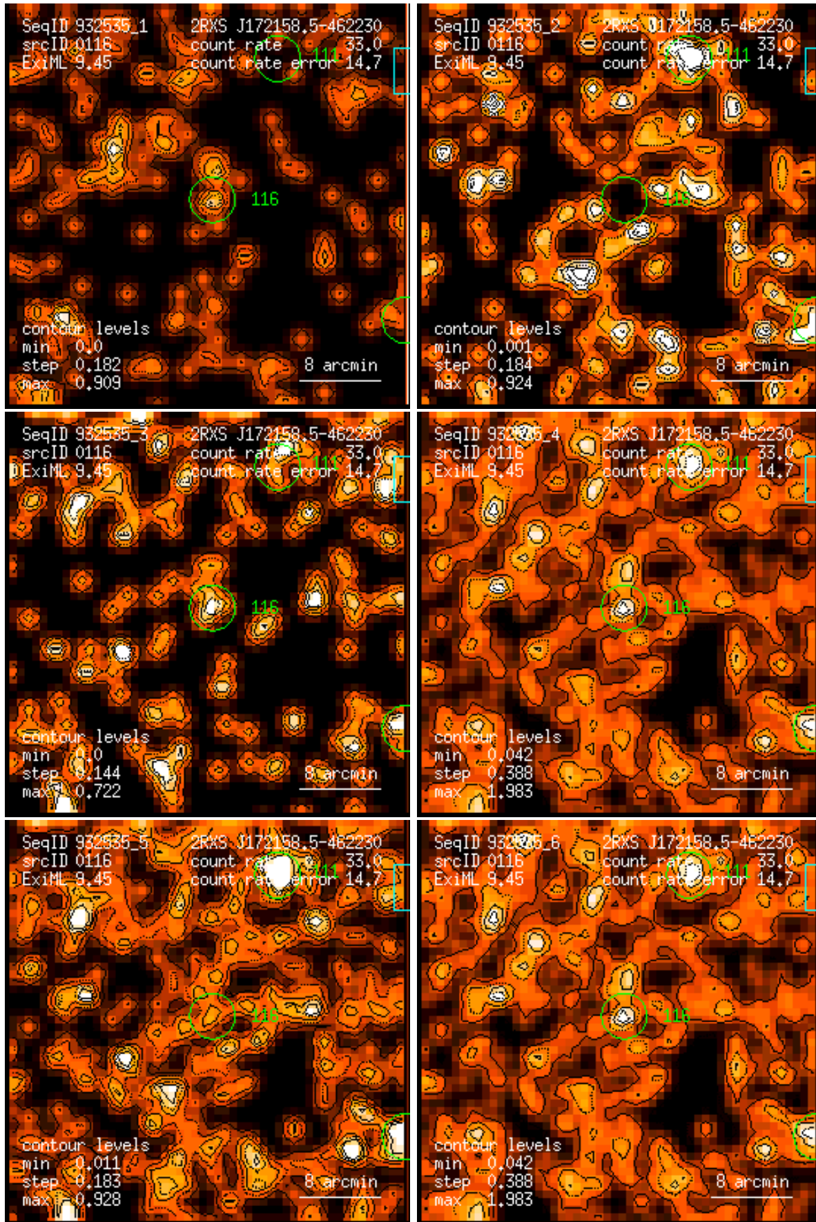
Figure 116: RASS 932535: detection 0116: band rate images, Gaussian filter: (1) PSPC channels 11 – 41, (2) 52 – 90, (3) 91 – 201, (4) 11 – 235, (5) 52 – 201, (6) 11 – 201. Broad band rates in counts/ks. Band rate contour levels in counts/ks/arcmin 2 .
