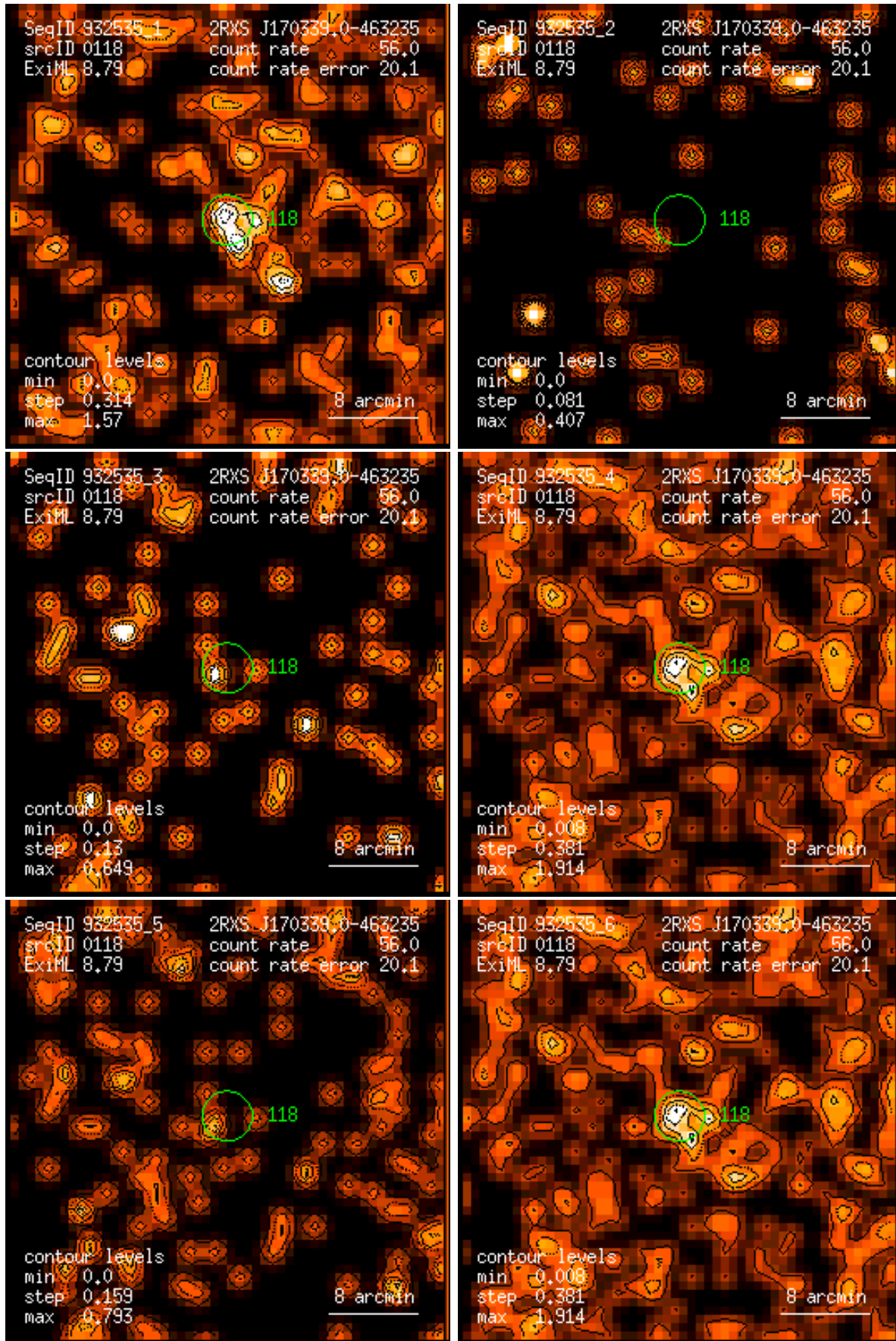
Figure 118: RASS 932535: detection 0118: band rate images, Gaussian filter: (1) PSPC channels 11 – 41, (2) 52 – 90, (3) 91 – 201, (4) 11 – 235, (5) 52 – 201, (6) 11 – 201. Broad band rates in counts/ks. Band rate contour levels in counts/ks/arcmin 2 .
