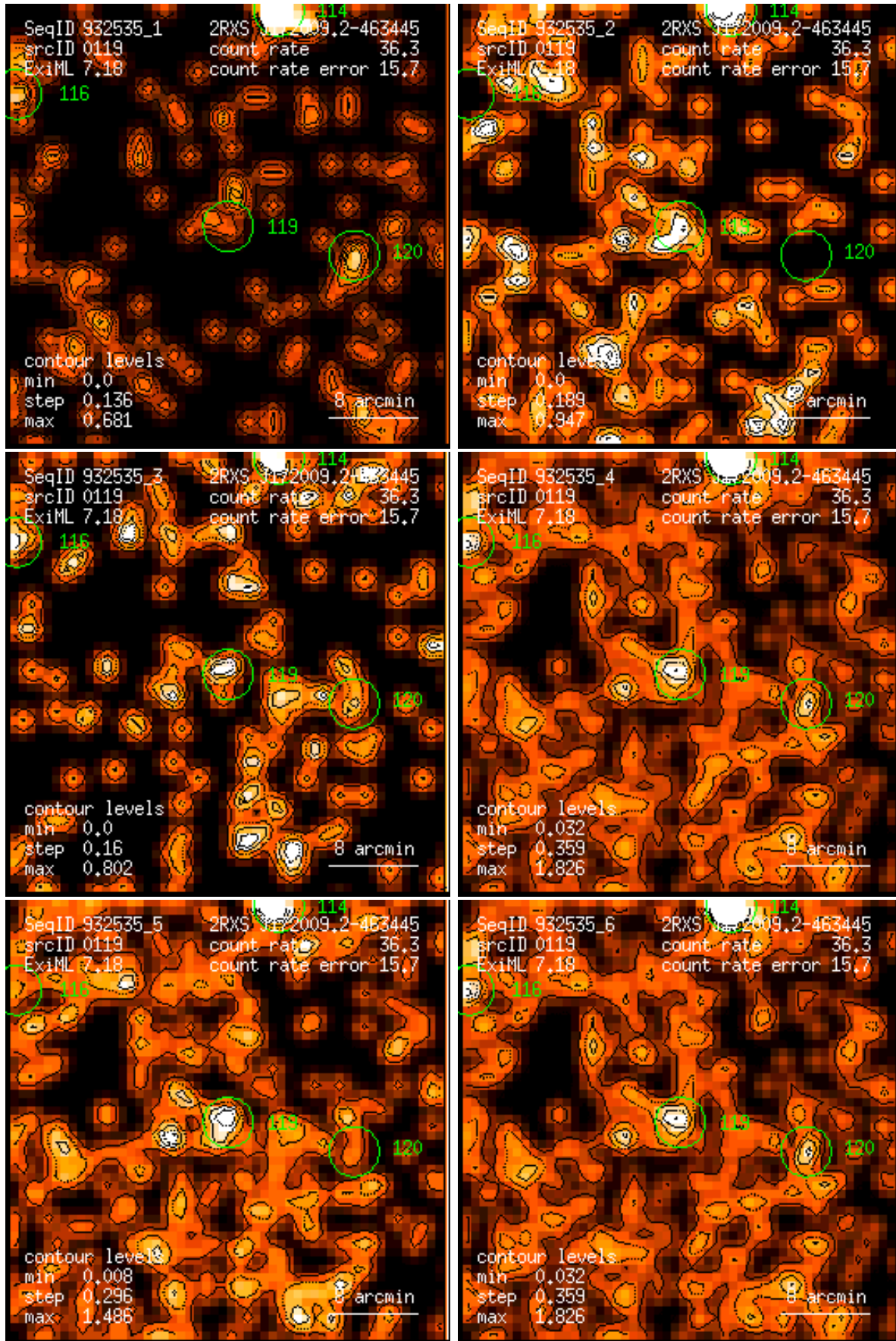
Figure 119: RASS 932535: detection 0119: band rate images, Gaussian filter: (1) PSPC channels 11 – 41, (2) 52 – 90, (3) 91 – 201, (4) 11 – 235, (5) 52 – 201, (6) 11 – 201. Broad band rates in counts/ks. Band rate contour levels in counts/ks/arcmin 2 .
