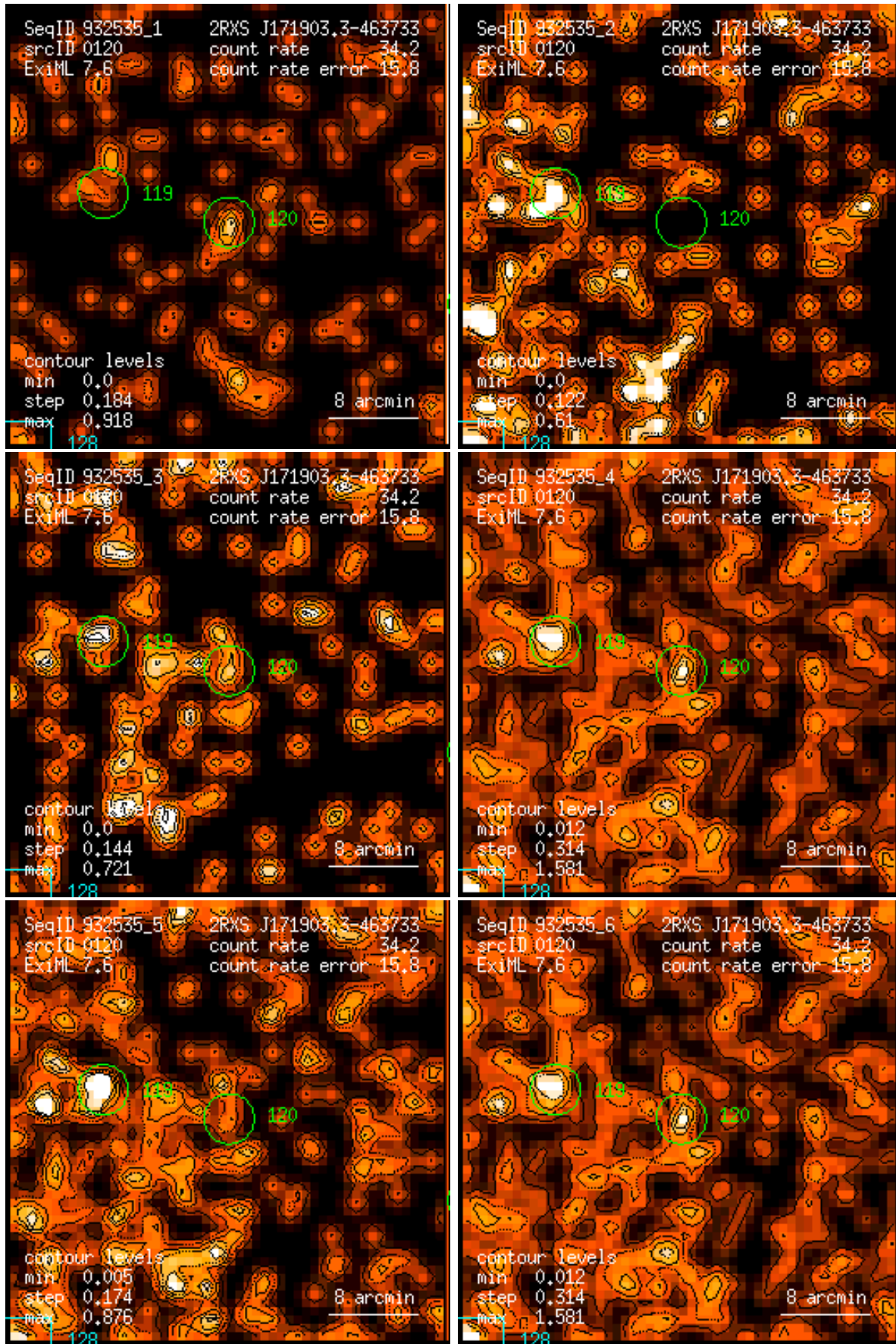
Figure 120: RASS 932535: detection 0120: band rate images, Gaussian filter: (1) PSPC channels 11 – 41, (2) 52 – 90, (3) 91 – 201, (4) 11 – 235, (5) 52 – 201, (6) 11 – 201. Broad band rates in counts/ks. Band rate contour levels in counts/ks/arcmin 2 .
