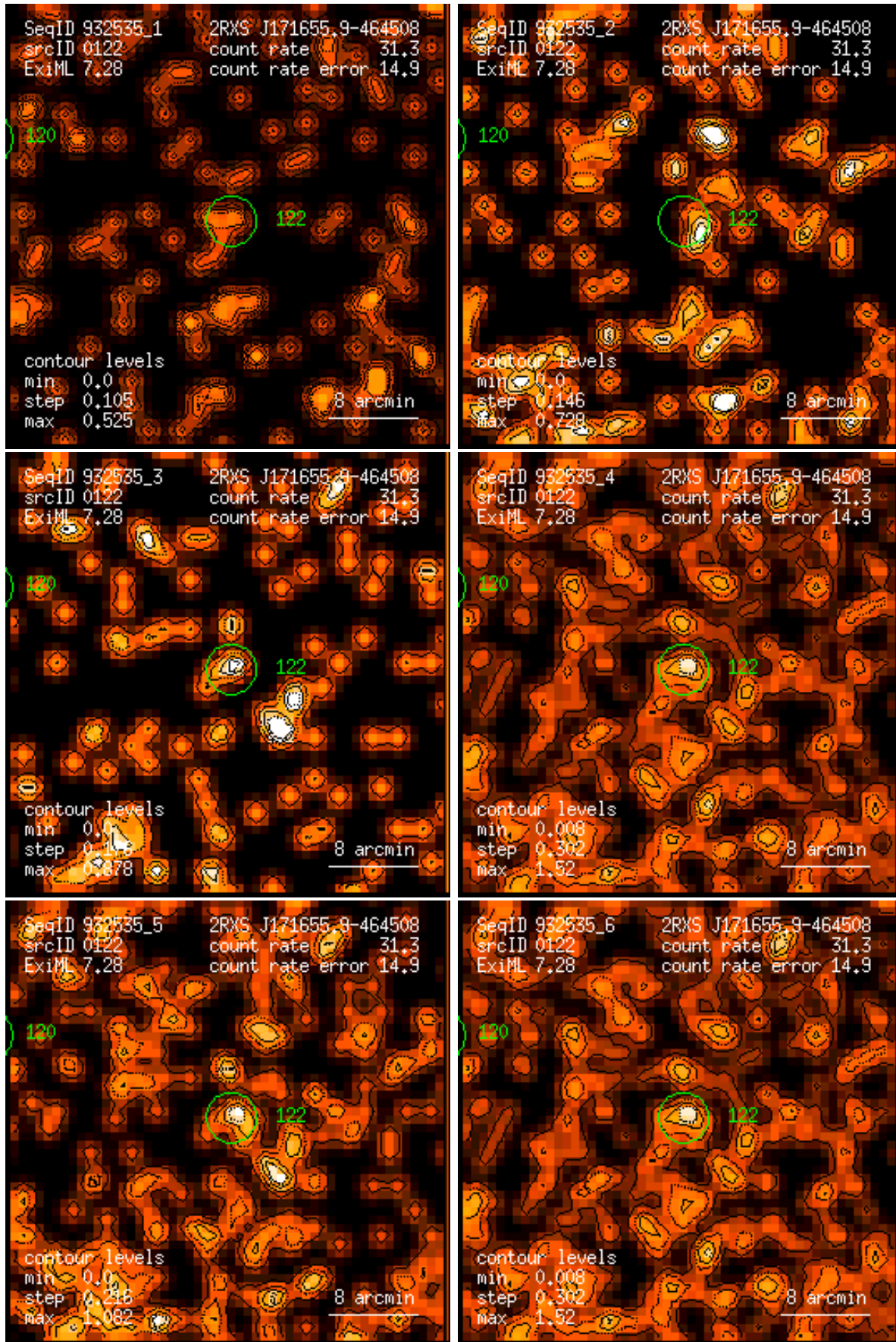
Figure 122: RASS 932535: detection 0122: band rate images, Gaussian filter: (1) PSPC channels 11 – 41, (2) 52 – 90, (3) 91 – 201, (4) 11 – 235, (5) 52 – 201, (6) 11 – 201. Broad band rates in counts/ks. Band rate contour levels in counts/ks/arcmin 2 .
