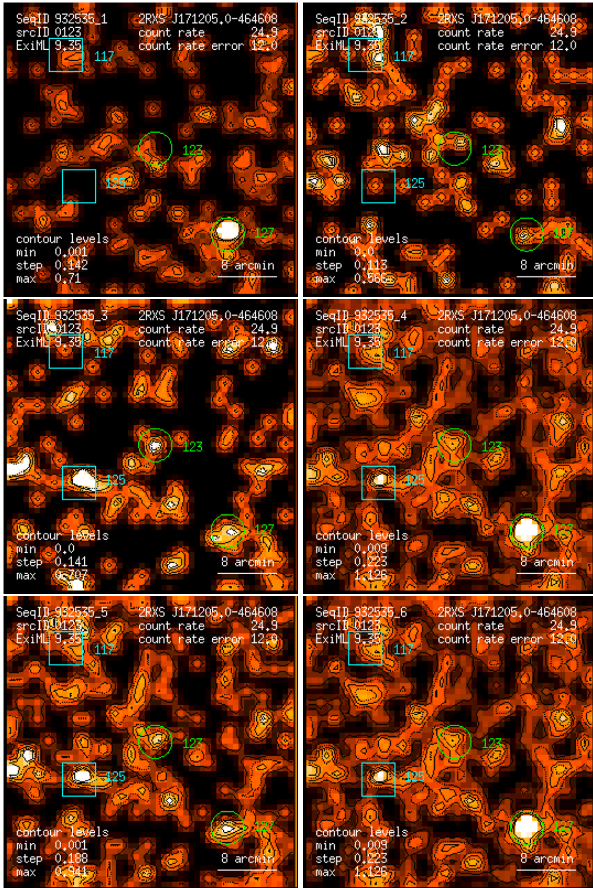
Figure 123: RASS 932535: detection 0123: band rate images, Gaussian filter: (1) PSPC channels 11 – 41, (2) 52 – 90, (3) 91 – 201, (4) 11 – 235, (5) 52 – 201, (6) 11 – 201. Broad band rates in counts/ks. Band rate contour levels in counts/ks/arcmin 2 .
