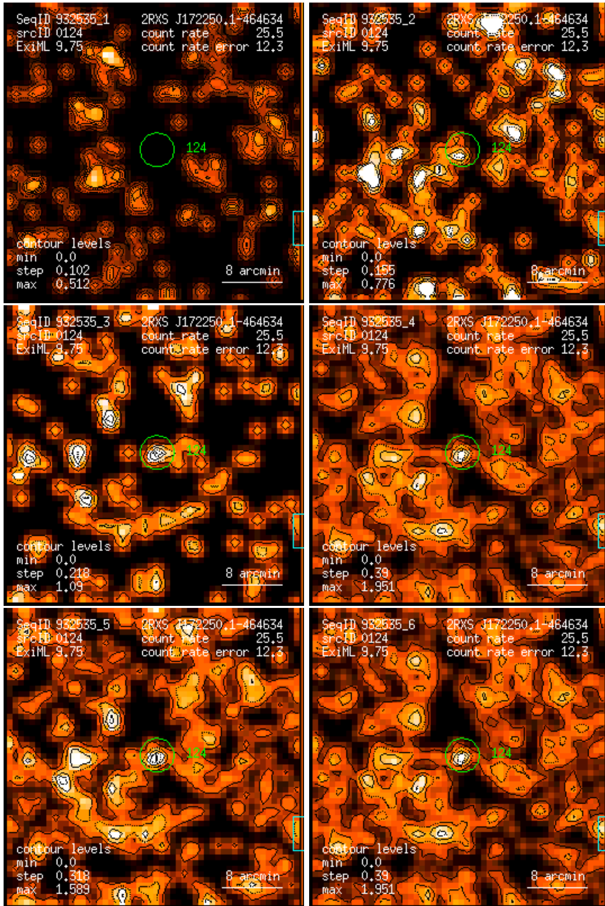
Figure 124: RASS 932535: detection 0124: band rate images, Gaussian filter: (1) PSPC channels 11 – 41, (2) 52 – 90, (3) 91 – 201, (4) 11 – 235, (5) 52 – 201, (6) 11 – 201. Broad band rates in counts/ks. Band rate contour levels in counts/ks/arcmin 2 .
