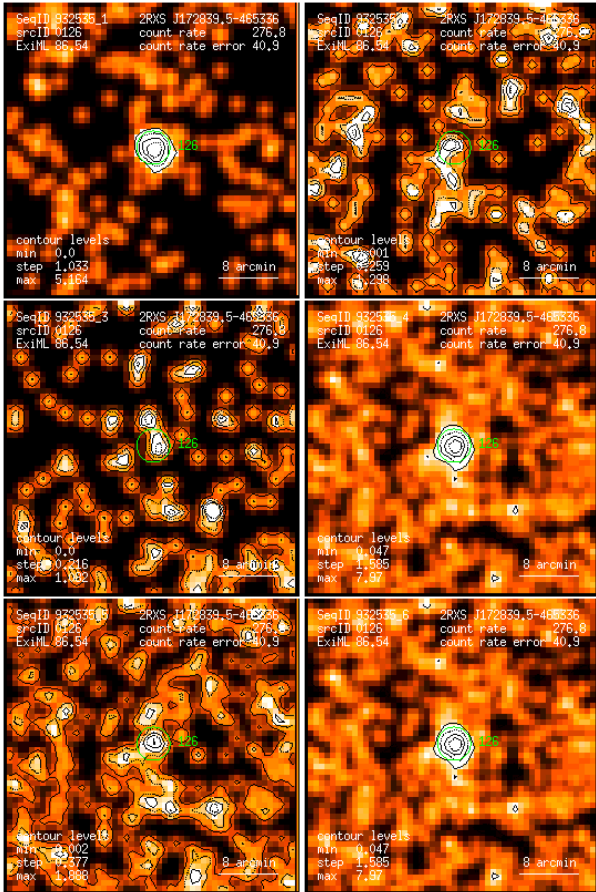
Figure 126: RASS 932535: detection 0126: band rate images, Gaussian filter: (1) PSPC channels 11 – 41, (2) 52 – 90, (3) 91 – 201, (4) 11 – 235, (5) 52 – 201, (6) 11 – 201. Broad band rates in counts/ks. Band rate contour levels in counts/ks/arcmin 2 .
