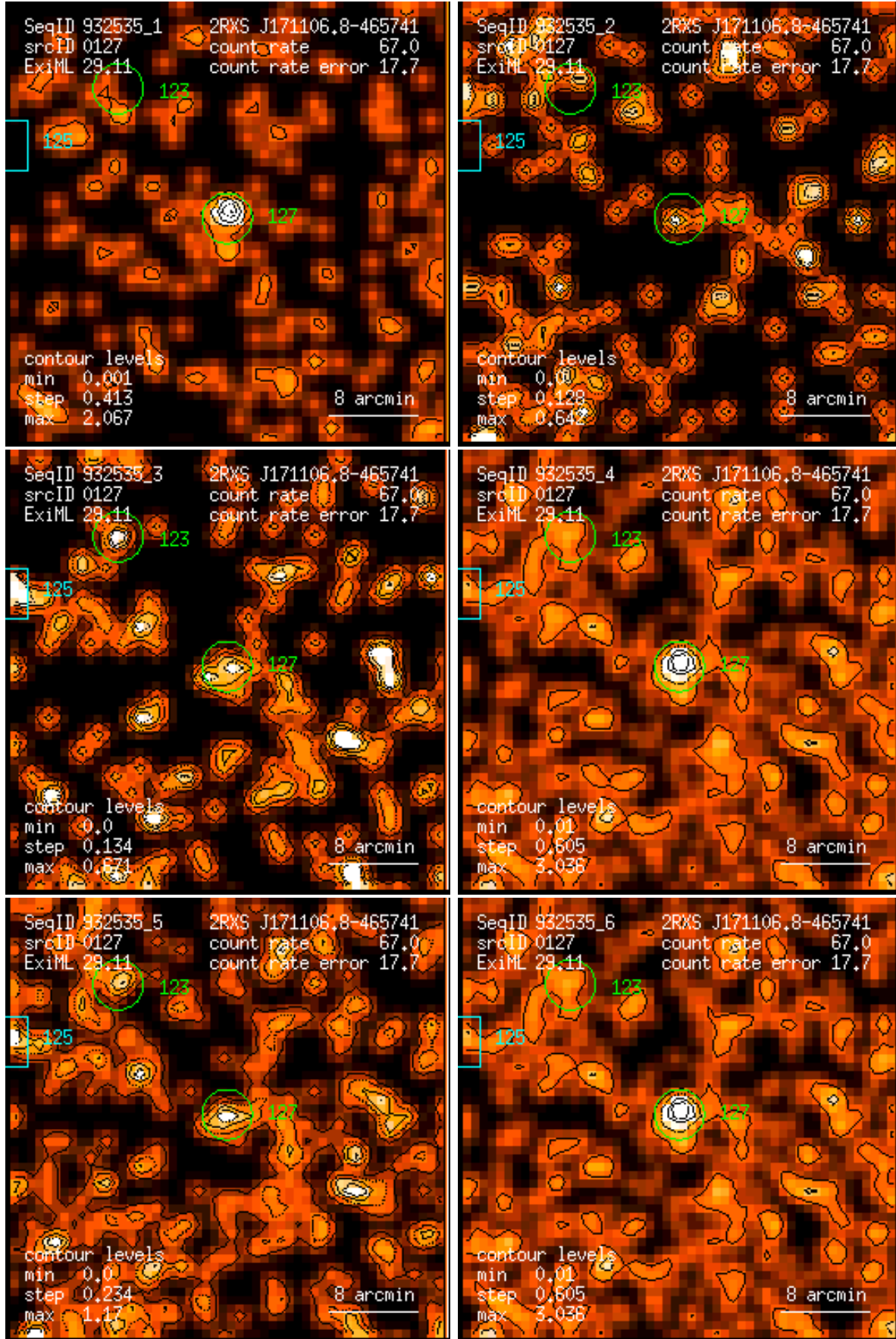
Figure 127: RASS 932535: detection 0127: band rate images, Gaussian filter: (1) PSPC channels 11 – 41, (2) 52 – 90, (3) 91 – 201, (4) 11 – 235, (5) 52 – 201, (6) 11 – 201. Broad band rates in counts/ks. Band rate contour levels in counts/ks/arcmin 2 .
