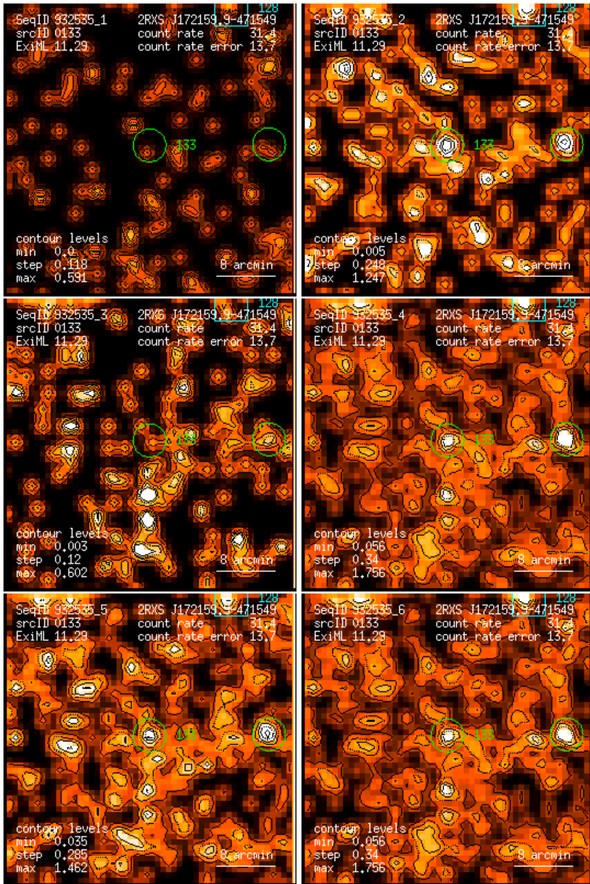
Figure 133: RASS 932535: detection 0133: band rate images, Gaussian filter: (1) PSPC channels 11 – 41, (2) 52 – 90, (3) 91 – 201, (4) 11 – 235, (5) 52 – 201, (6) 11 – 201. Broad band rates in counts/ks. Band rate contour levels in counts/ks/arcmin 2 .
