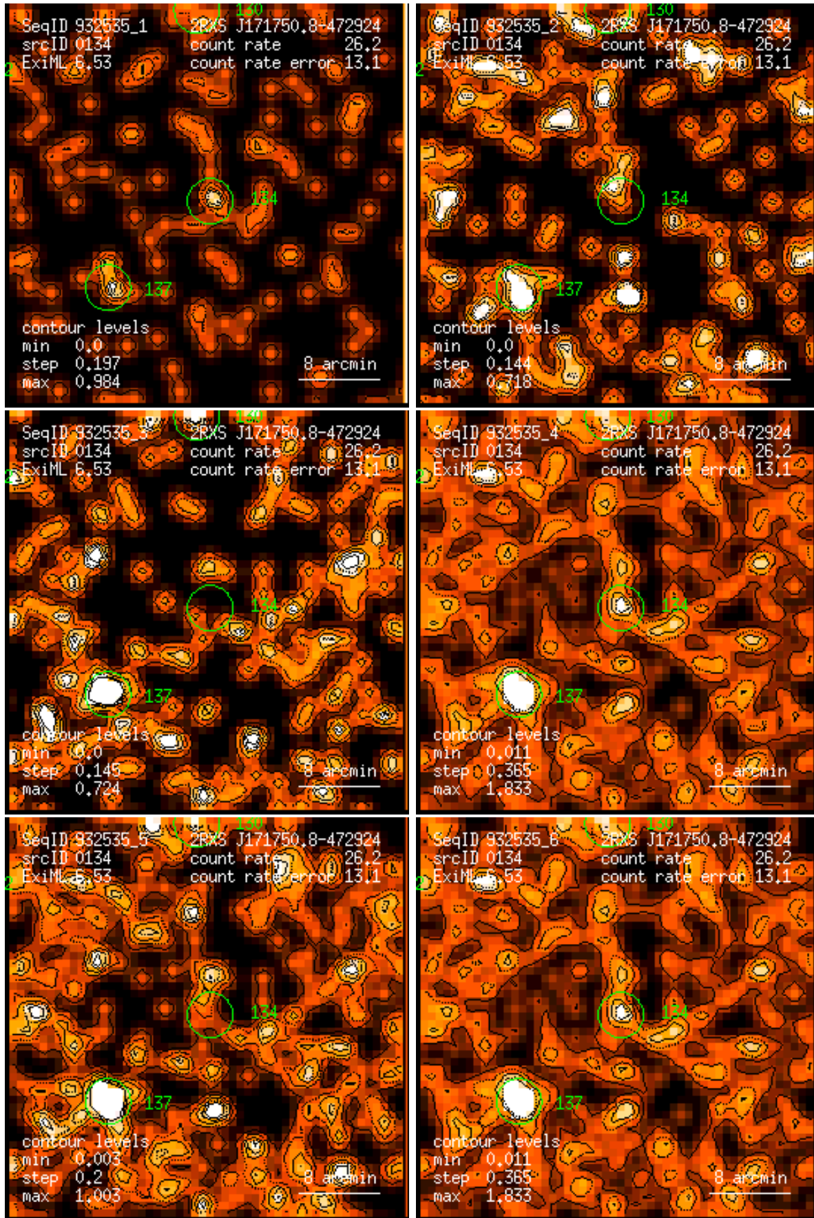
Figure 134: RASS 932535: detection 0134: band rate images, Gaussian filter: (1) PSPC channels 11 – 41, (2) 52 – 90, (3) 91 – 201, (4) 11 – 235, (5) 52 – 201, (6) 11 – 201. Broad band rates in counts/ks. Band rate contour levels in counts/ks/arcmin 2 .
