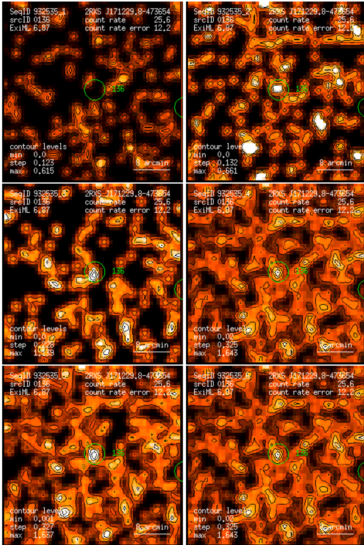
Figure 136: RASS 932535: detection 0136: band rate images, Gaussian filter: (1) PSPC channels 11 – 41, (2) 52 – 90, (3) 91 – 201, (4) 11 – 235, (5) 52 – 201, (6) 11 – 201. Broad band rates in counts/ks. Band rate contour levels in counts/ks/arcmin 2 .
