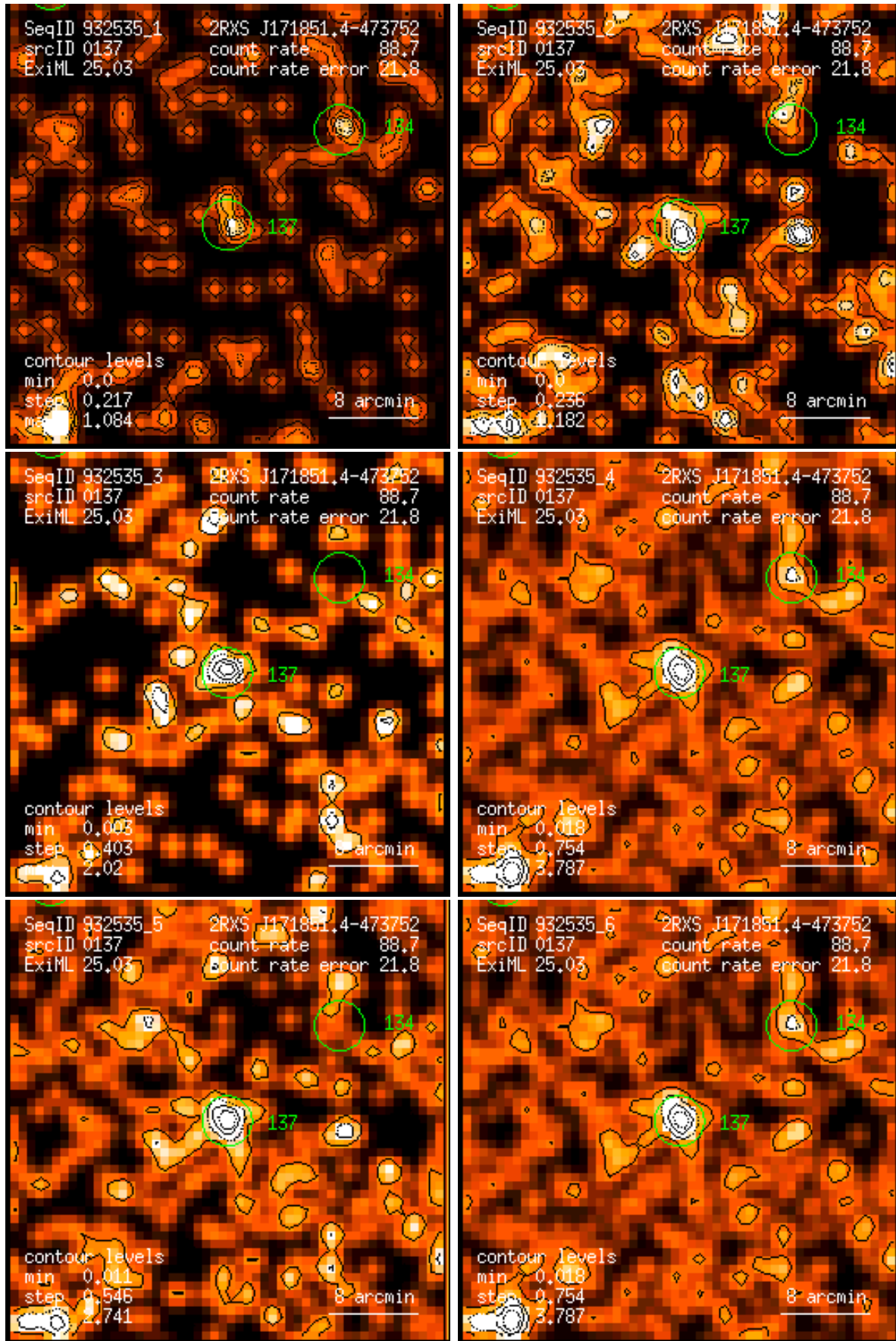
Figure 137: RASS 932535: detection 0137: band rate images, Gaussian filter: (1) PSPC channels 11 – 41, (2) 52 – 90, (3) 91 – 201, (4) 11 – 235, (5) 52 – 201, (6) 11 – 201. Broad band rates in counts/ks. Band rate contour levels in counts/ks/arcmin 2 .
