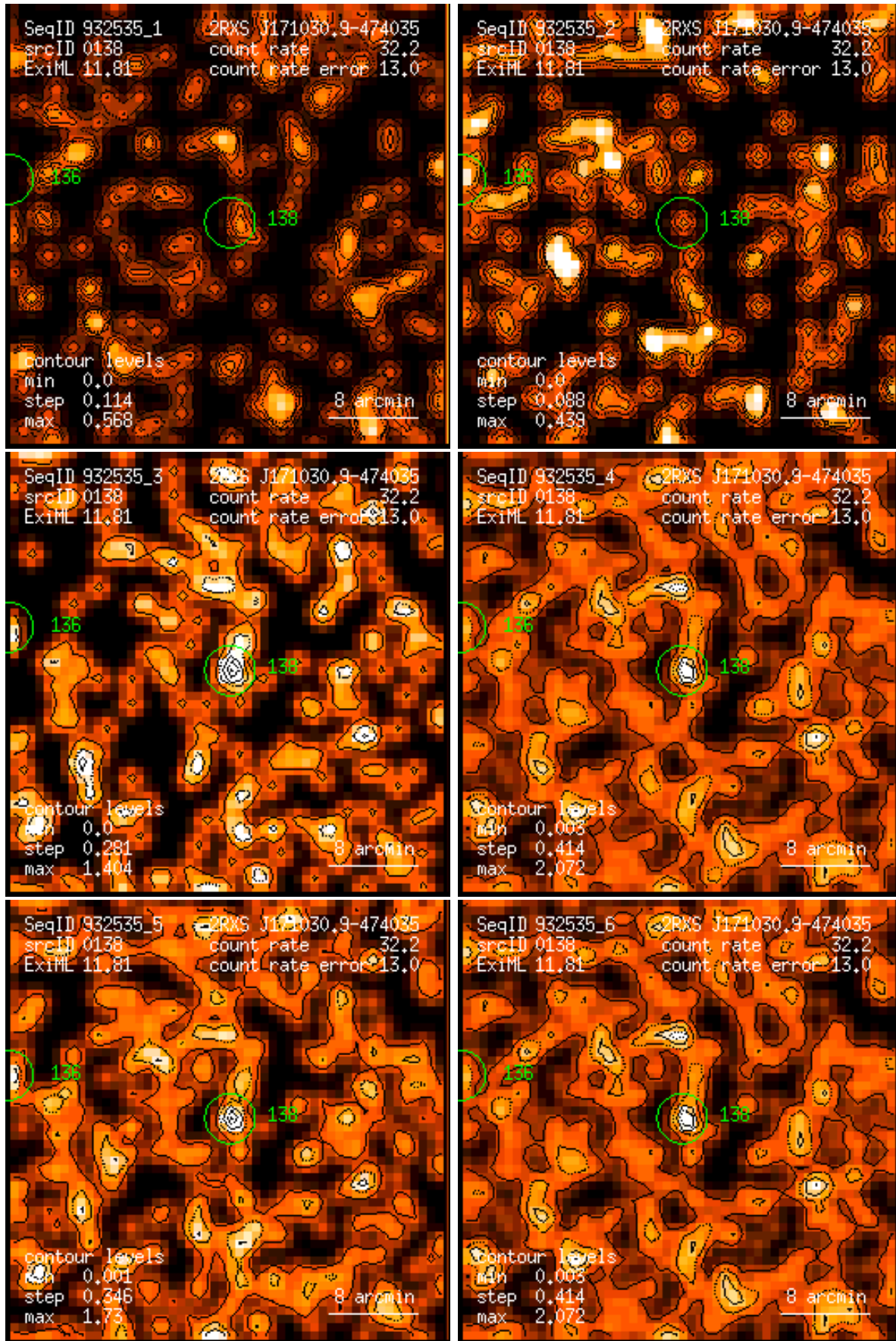
Figure 138: RASS 932535: detection 0138: band rate images, Gaussian filter: (1) PSPC channels 11 – 41, (2) 52 – 90, (3) 91 – 201, (4) 11 – 235, (5) 52 – 201, (6) 11 – 201. Broad band rates in counts/ks. Band rate contour levels in counts/ks/arcmin 2 .
