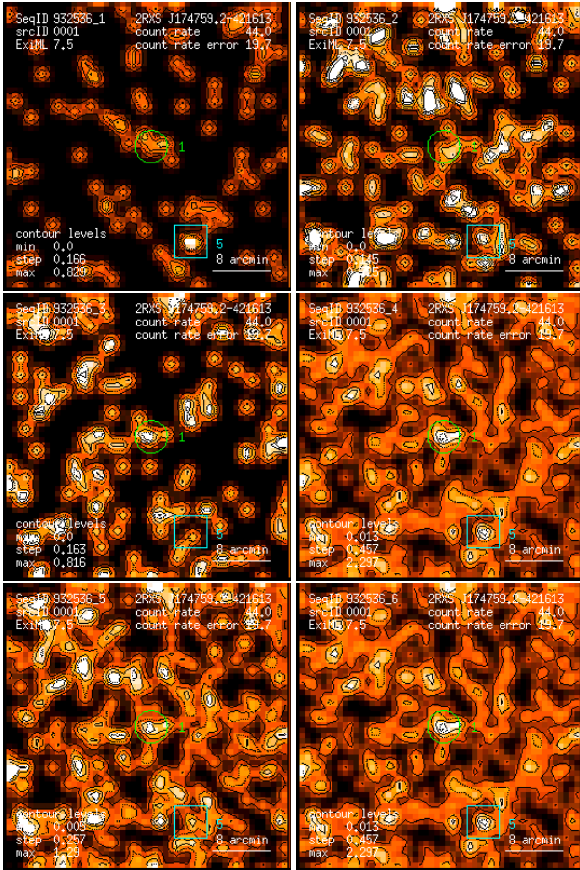
Figure 1: RASS 932536: detection 0001: band rate images, Gaussian filter: (1) PSPC channels 11 – 41, (2) 52 – 90, (3) 91 – 201, (4) 11 – 235, (5) 52 – 201, (6) 11 – 201. Broad band rates in counts/ks. Band rate contour levels in counts/ks/arcmin 2 .
