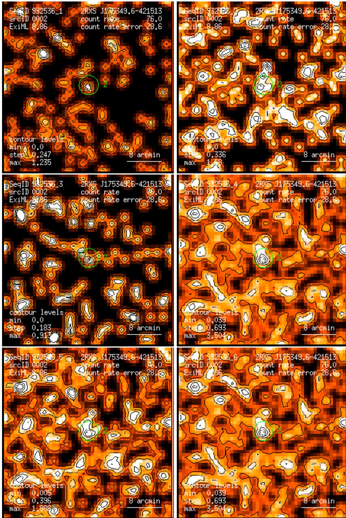
Figure 2: RASS 932536: detection 0002: band rate images, Gaussian filter: (1) PSPC channels 11 – 41, (2) 52 – 90, (3) 91 – 201, (4) 11 – 235, (5) 52 – 201, (6) 11 – 201. Broad band rates in counts/ks. Band rate contour levels in counts/ks/arcmin 2 .
