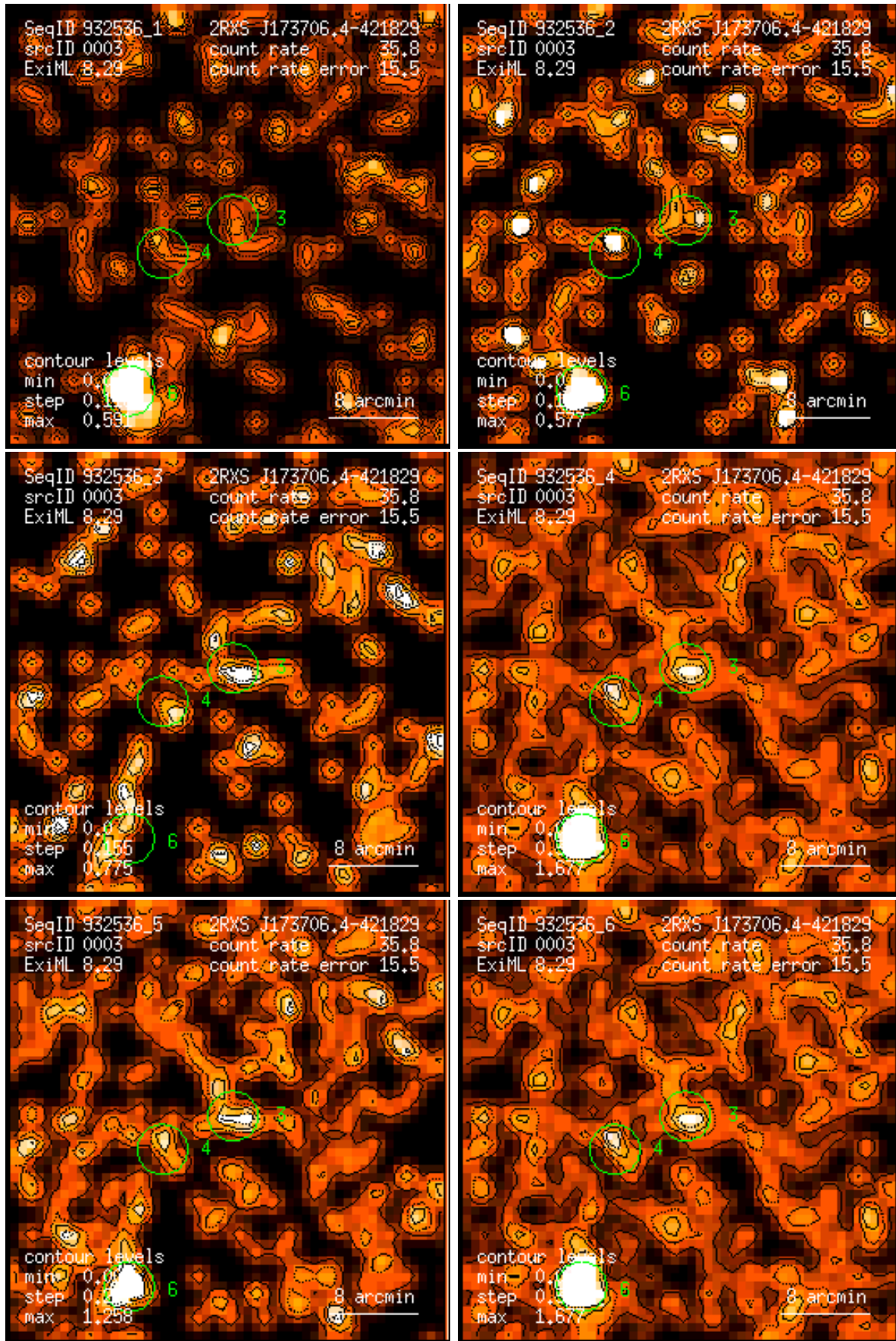
Figure 3: RASS 932536: detection 0003: band rate images, Gaussian filter: (1) PSPC channels 11 – 41, (2) 52 – 90, (3) 91 – 201, (4) 11 – 235, (5) 52 – 201, (6) 11 – 201. Broad band rates in counts/ks. Band rate contour levels in counts/ks/arcmin 2 .
