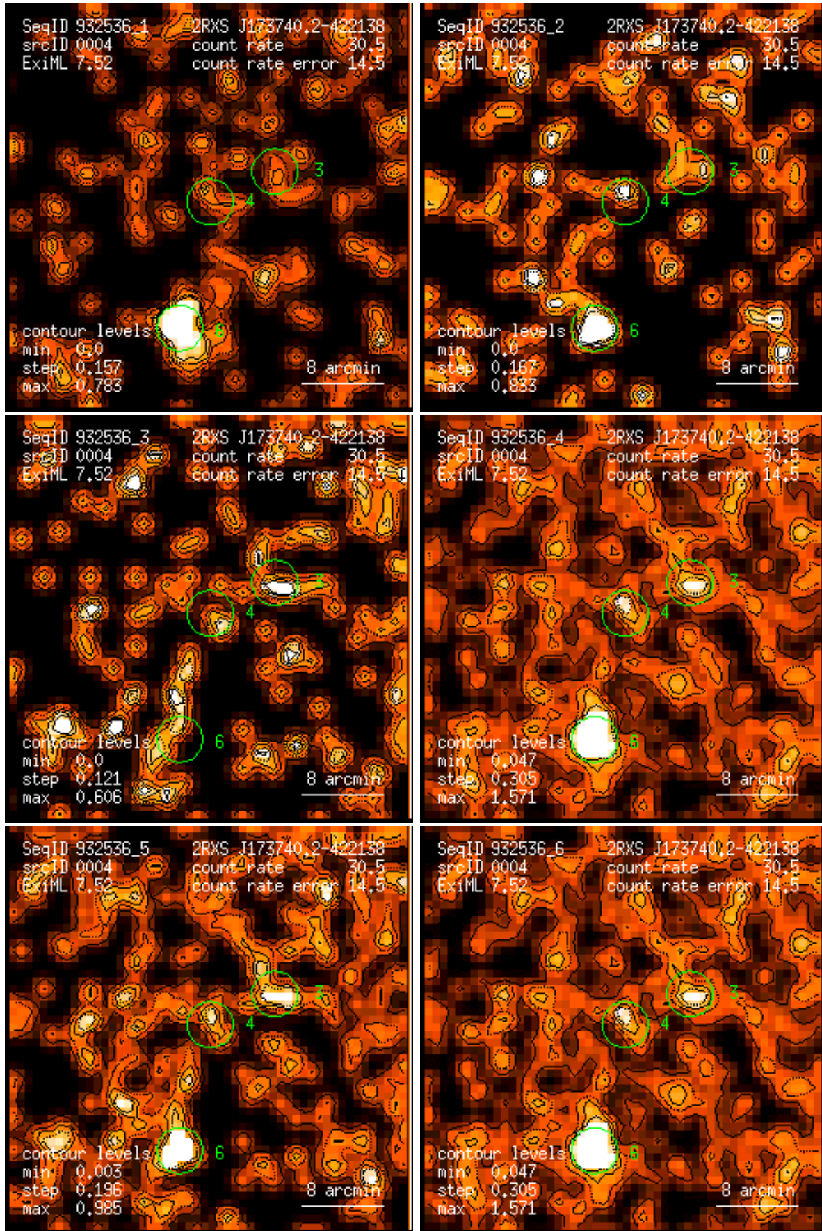
Figure 4: RASS 932536: detection 0004: band rate images, Gaussian filter: (1) PSPC channels 11 – 41, (2) 52 – 90, (3) 91 – 201, (4) 11 – 235, (5) 52 – 201, (6) 11 – 201. Broad band rates in counts/ks. Band rate contour levels in counts/ks/arcmin 2 .
