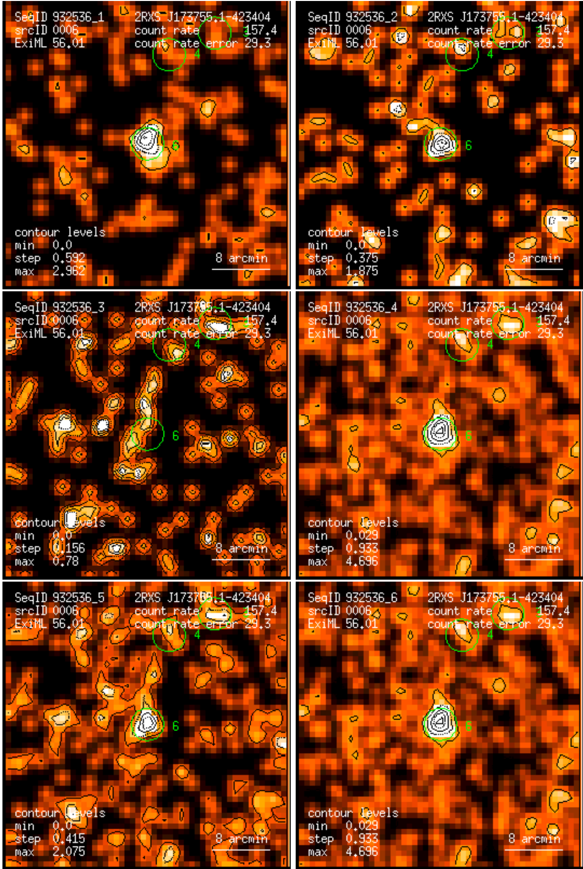
Figure 6: RASS 932536: detection 0006: band rate images, Gaussian filter: (1) PSPC channels 11 – 41, (2) 52 – 90, (3) 91 – 201, (4) 11 – 235, (5) 52 – 201, (6) 11 – 201. Broad band rates in counts/ks. Band rate contour levels in counts/ks/arcmin 2 .
