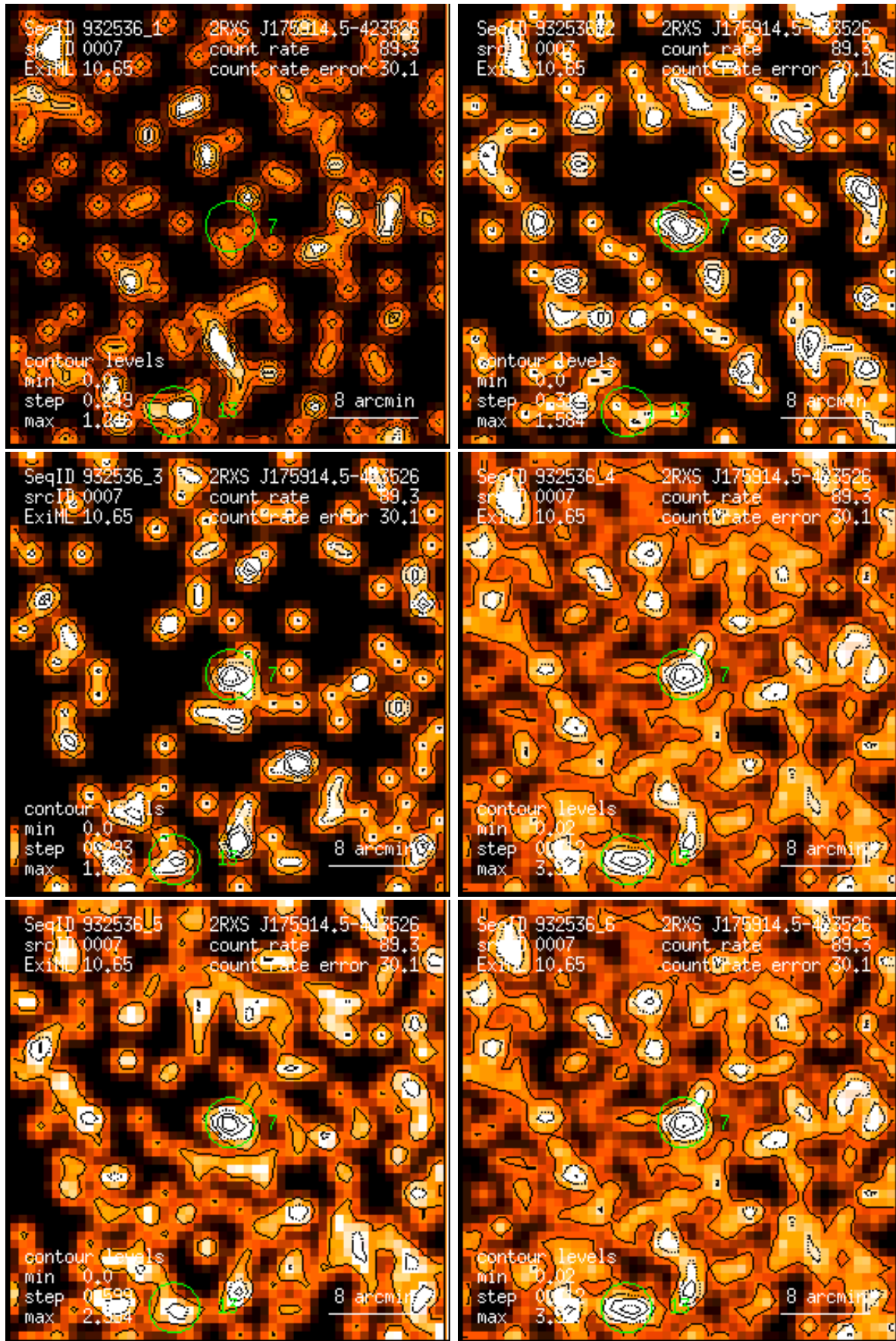
Figure 7: RASS 932536: detection 0007: band rate images, Gaussian filter: (1) PSPC channels 11 – 41, (2) 52 – 90, (3) 91 – 201, (4) 11 – 235, (5) 52 – 201, (6) 11 – 201. Broad band rates in counts/ks. Band rate contour levels in counts/ks/arcmin 2 .
