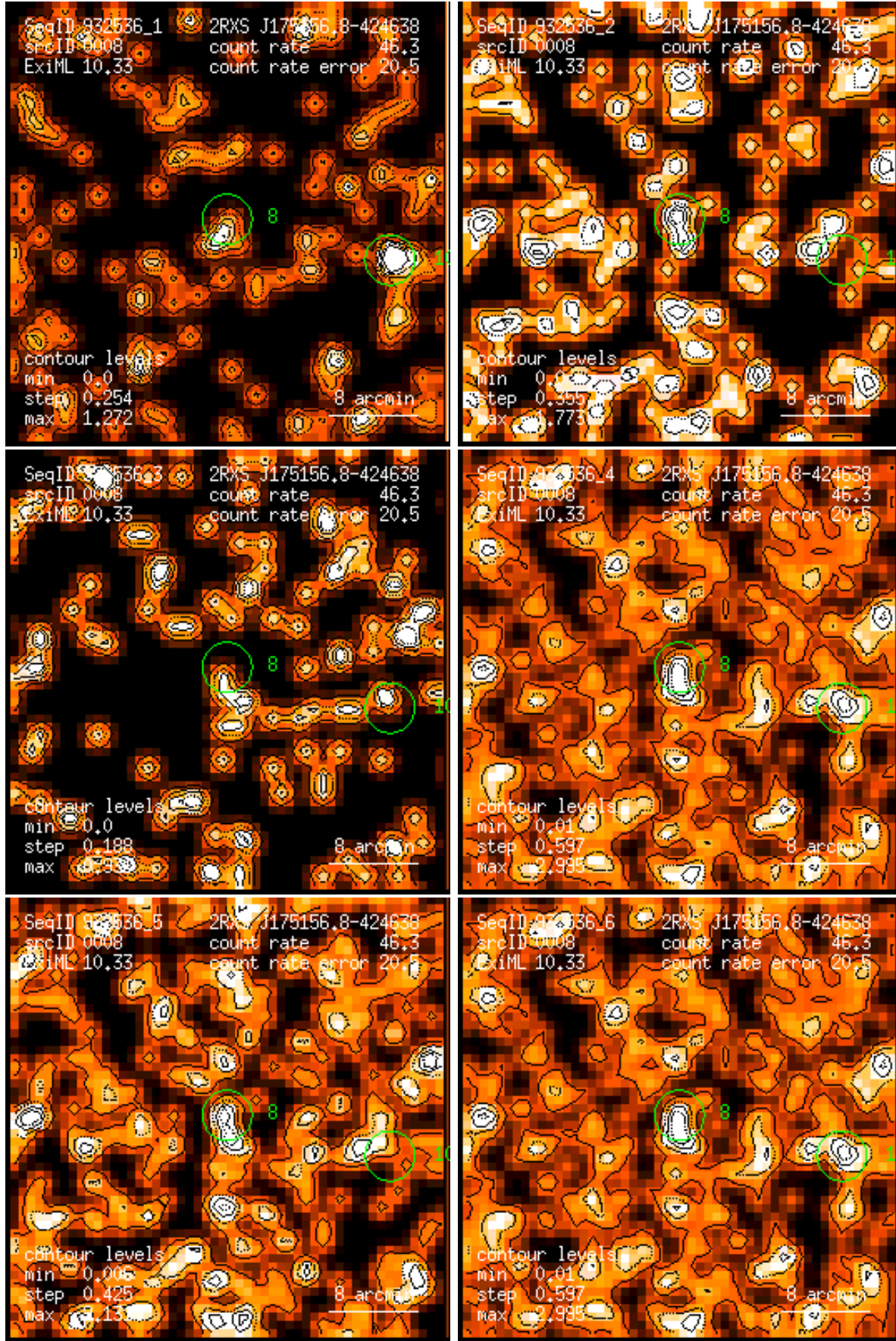
Figure 8: RASS 932536: detection 0008: band rate images, Gaussian filter: (1) PSPC channels 11 – 41, (2) 52 – 90, (3) 91 – 201, (4) 11 – 235, (5) 52 – 201, (6) 11 – 201. Broad band rates in counts/ks. Band rate contour levels in counts/ks/arcmin 2 .
