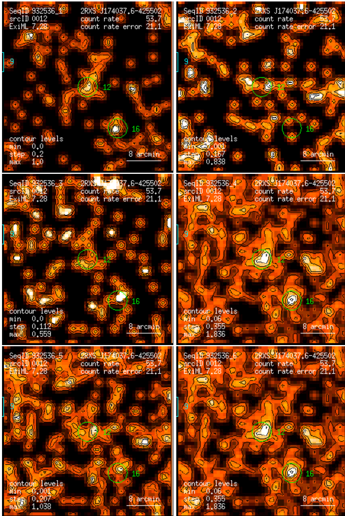
Figure 12: RASS 932536: detection 0012: band rate images, Gaussian filter: (1) PSPC channels 11 – 41, (2) 52 – 90, (3) 91 – 201, (4) 11 – 235, (5) 52 – 201, (6) 11 – 201. Broad band rates in counts/ks. Band rate contour levels in counts/ks/arcmin 2 .
