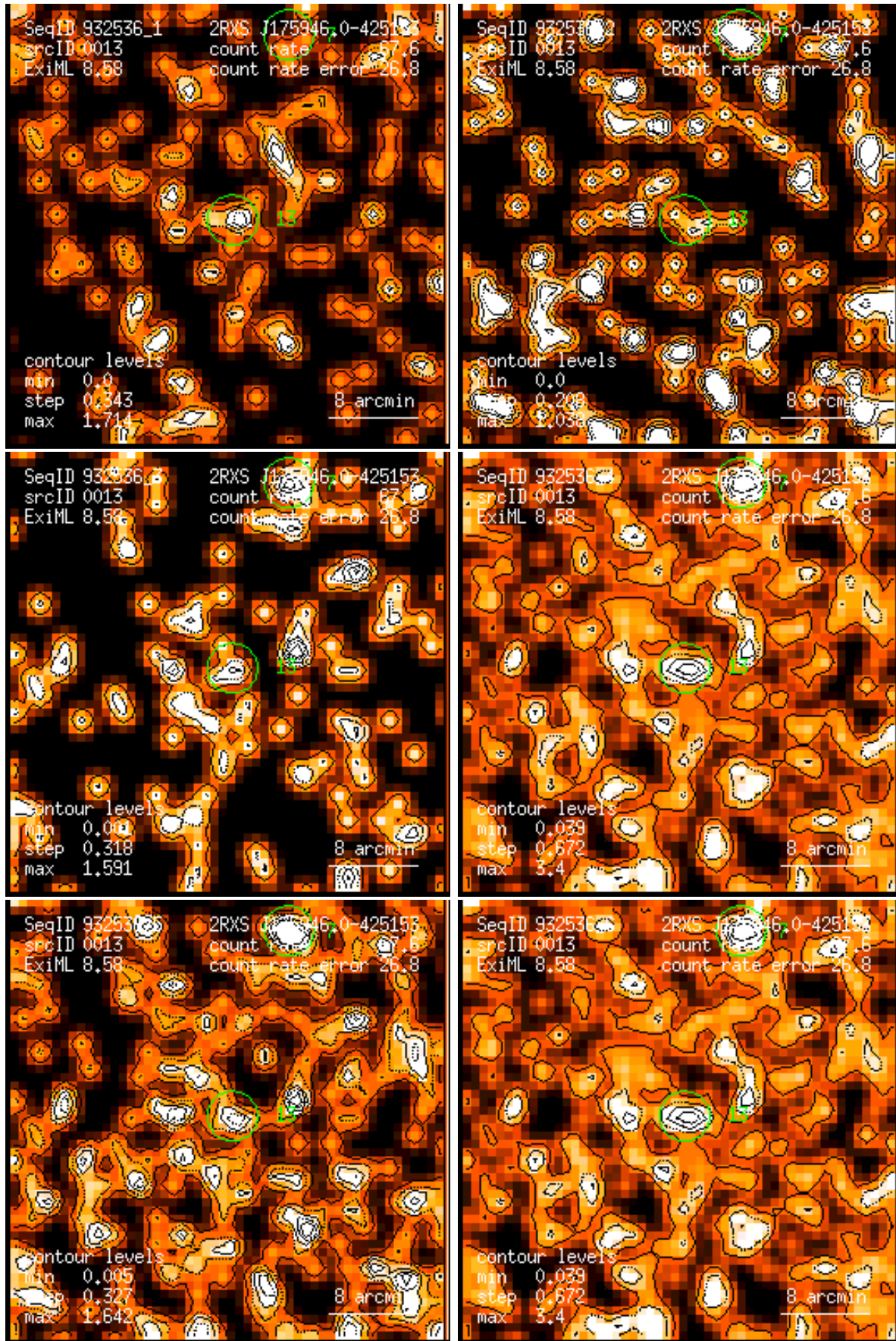
Figure 13: RASS 932536: detection 0013: band rate images, Gaussian filter: (1) PSPC channels 11 – 41, (2) 52 – 90, (3) 91 – 201, (4) 11 – 235, (5) 52 – 201, (6) 11 – 201. Broad band rates in counts/ks. Band rate contour levels in counts/ks/arcmin 2 .
