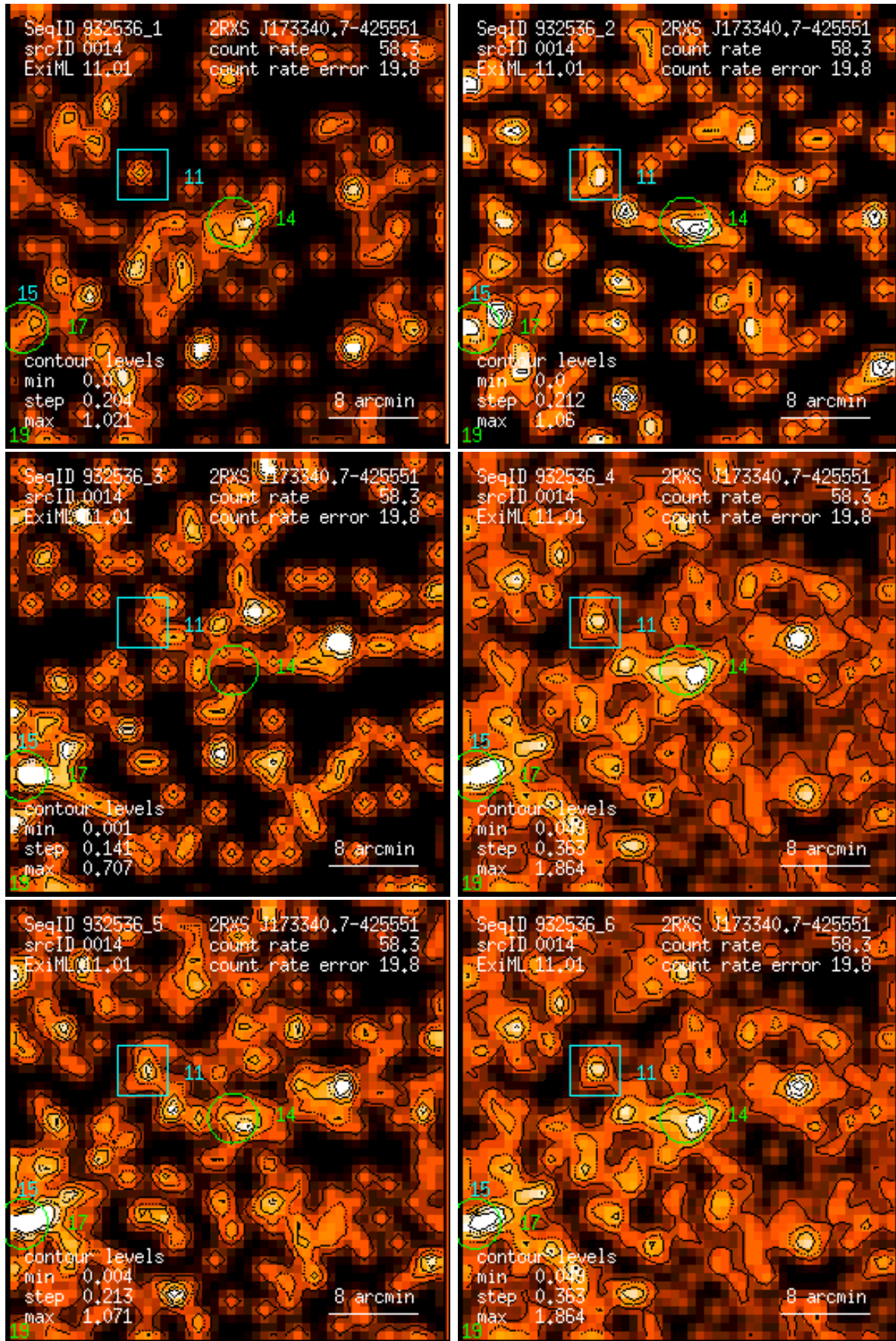
Figure 14: RASS 932536: detection 0014: band rate images, Gaussian filter: (1) PSPC channels 11 – 41, (2) 52 – 90, (3) 91 – 201, (4) 11 – 235, (5) 52 – 201, (6) 11 – 201. Broad band rates in counts/ks. Band rate contour levels in counts/ks/arcmin 2 .
