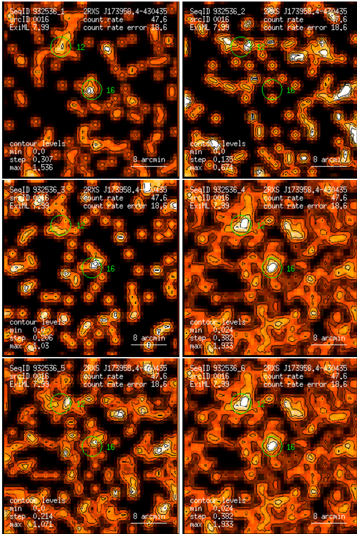
Figure 16: RASS 932536: detection 0016: band rate images, Gaussian filter: (1) PSPC channels 11 – 41, (2) 52 – 90, (3) 91 – 201, (4) 11 – 235, (5) 52 – 201, (6) 11 – 201. Broad band rates in counts/ks. Band rate contour levels in counts/ks/arcmin 2 .
