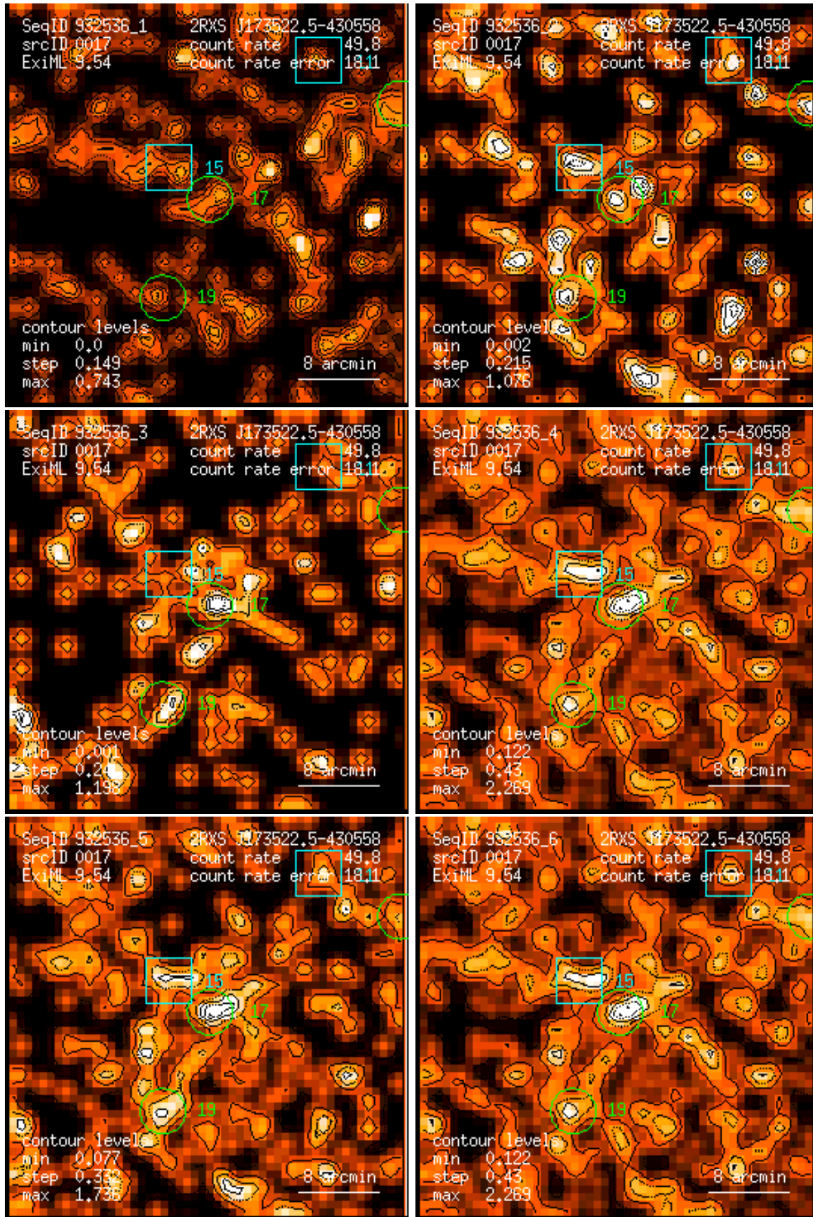
Figure 17: RASS 932536: detection 0017: band rate images, Gaussian filter: (1) PSPC channels 11 – 41, (2) 52 – 90, (3) 91 – 201, (4) 11 – 235, (5) 52 – 201, (6) 11 – 201. Broad band rates in counts/ks. Band rate contour levels in counts/ks/arcmin 2 .
