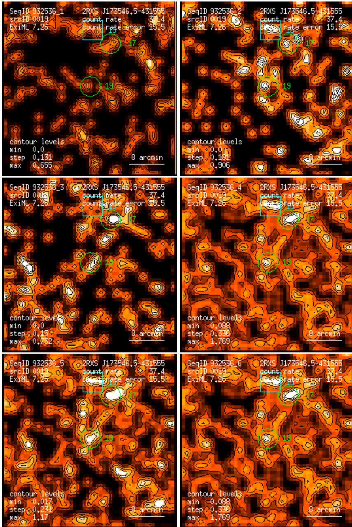
Figure 19: RASS 932536: detection 0019: band rate images, Gaussian filter: (1) PSPC channels 11 – 41, (2) 52 – 90, (3) 91 – 201, (4) 11 – 235, (5) 52 – 201, (6) 11 – 201. Broad band rates in counts/ks. Band rate contour levels in counts/ks/arcmin 2 .
