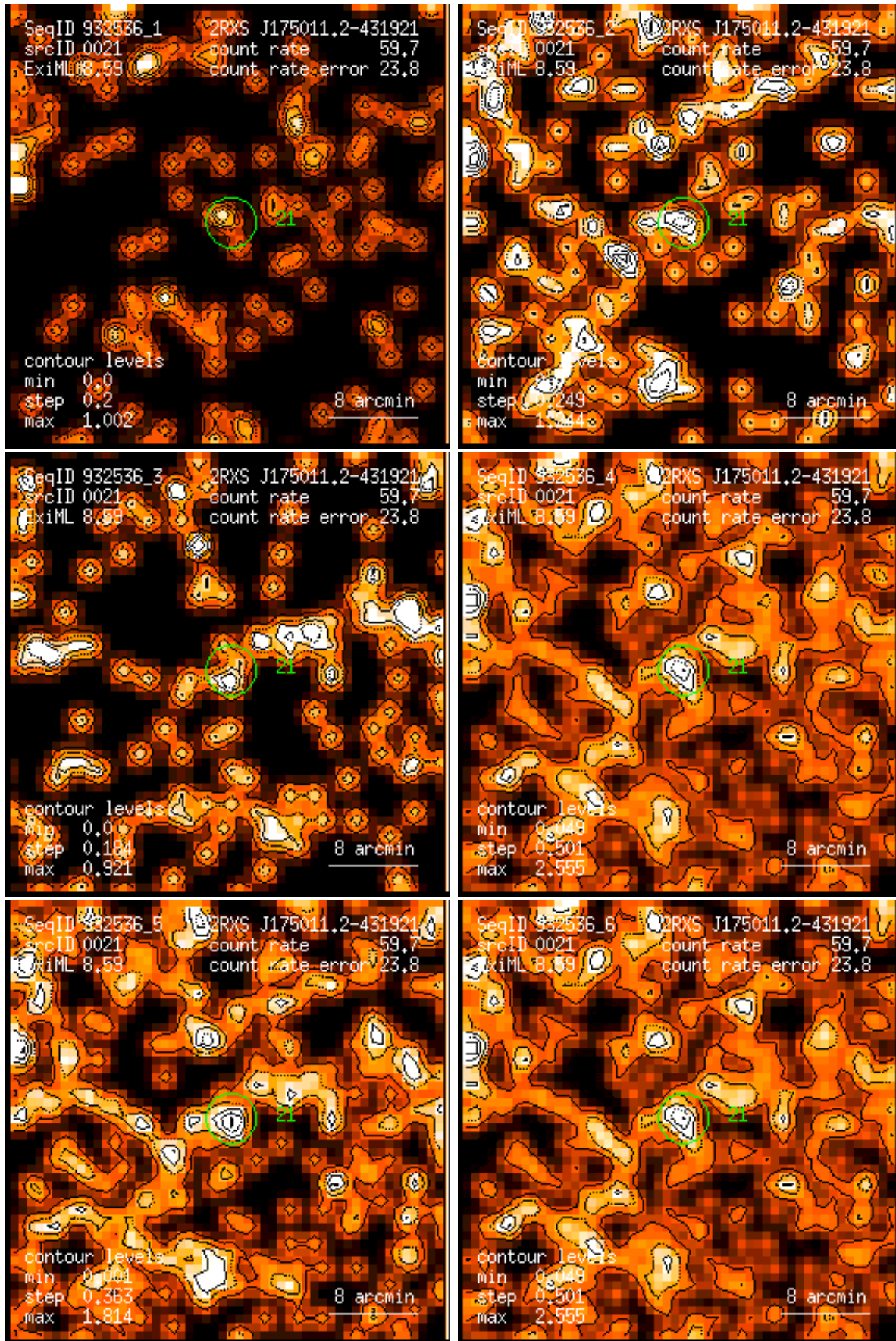
Figure 21: RASS 932536: detection 0021: band rate images, Gaussian filter: (1) PSPC channels 11 – 41, (2) 52 – 90, (3) 91 – 201, (4) 11 – 235, (5) 52 – 201, (6) 11 – 201. Broad band rates in counts/ks. Band rate contour levels in counts/ks/arcmin 2 .
