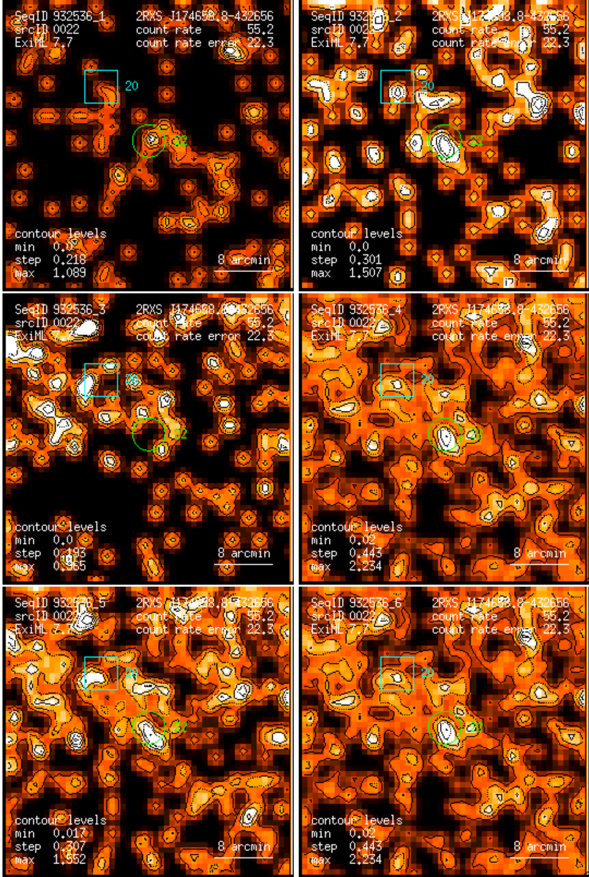
Figure 22: RASS 932536: detection 0022: band rate images, Gaussian filter: (1) PSPC channels 11 – 41, (2) 52 – 90, (3) 91 – 201, (4) 11 – 235, (5) 52 – 201, (6) 11 – 201. Broad band rates in counts/ks. Band rate contour levels in counts/ks/arcmin 2 .
