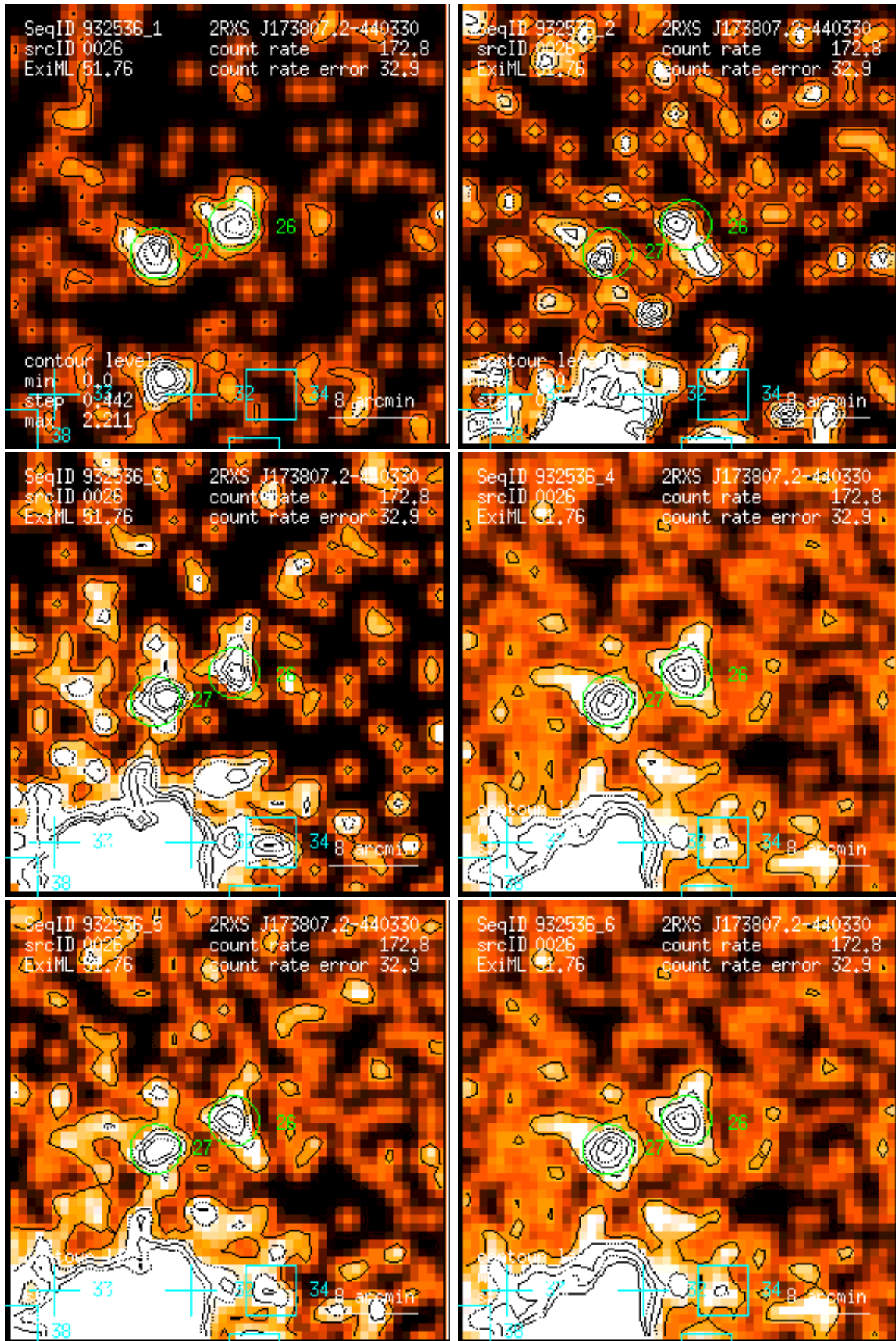
Figure 26: RASS 932536: detection 0026: band rate images, Gaussian filter: (1) PSPC channels 11 – 41, (2) 52 – 90, (3) 91 – 201, (4) 11 – 235, (5) 52 – 201, (6) 11 – 201. Broad band rates in counts/ks. Band rate contour levels in counts/ks/arcmin 2 .
