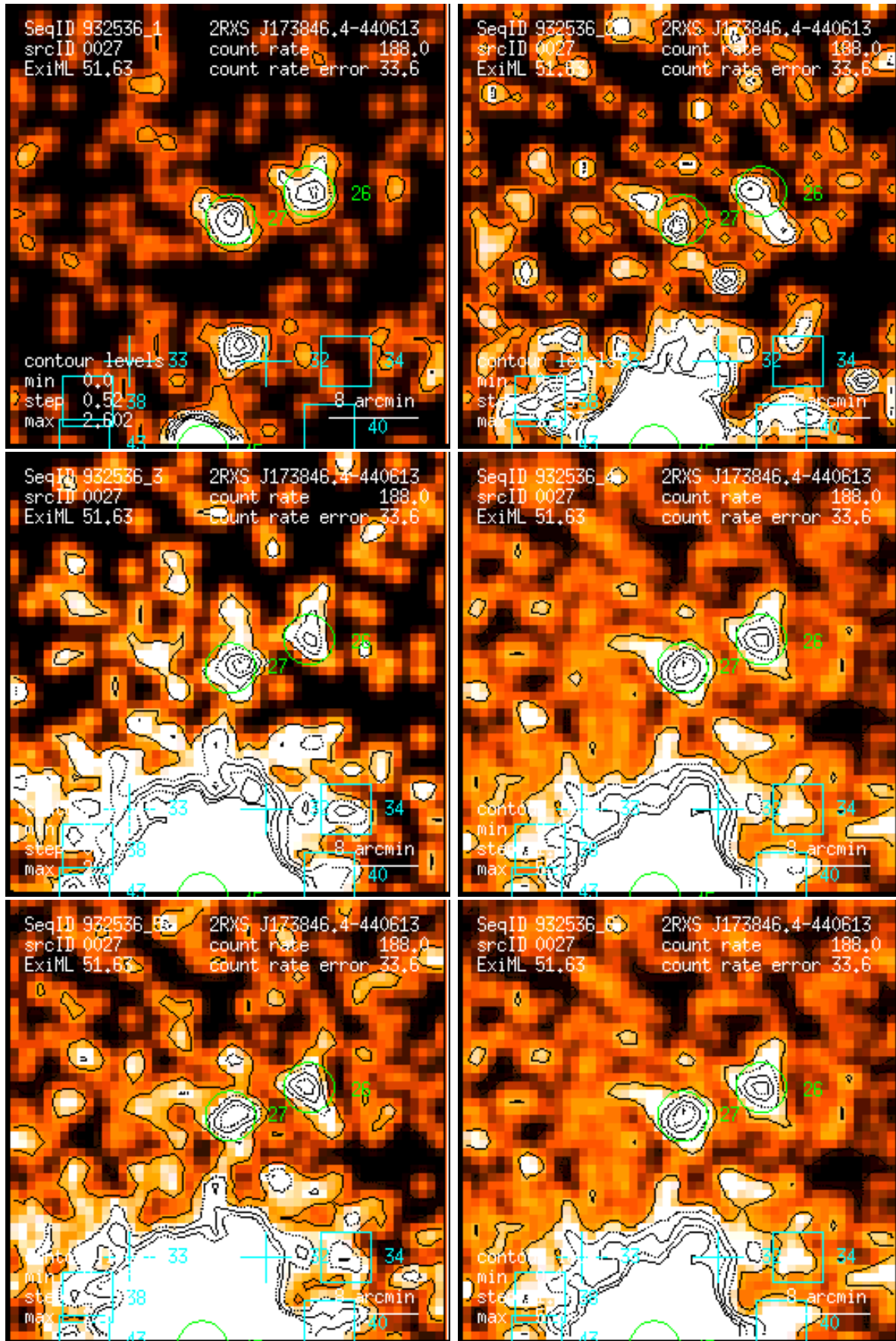
Figure 27: RASS 932536: detection 0027: band rate images, Gaussian filter: (1) PSPC channels 11 – 41, (2) 52 – 90, (3) 91 – 201, (4) 11 – 235, (5) 52 – 201, (6) 11 – 201. Broad band rates in counts/ks. Band rate contour levels in counts/ks/arcmin 2 .
