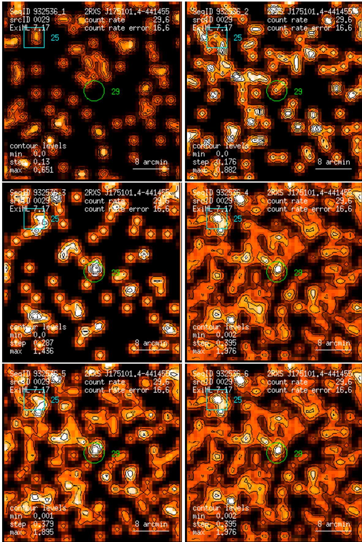
Figure 29: RASS 932536: detection 0029: band rate images, Gaussian filter: (1) PSPC channels 11 – 41, (2) 52 – 90, (3) 91 – 201, (4) 11 – 235, (5) 52 – 201, (6) 11 – 201. Broad band rates in counts/ks. Band rate contour levels in counts/ks/arcmin 2 .
