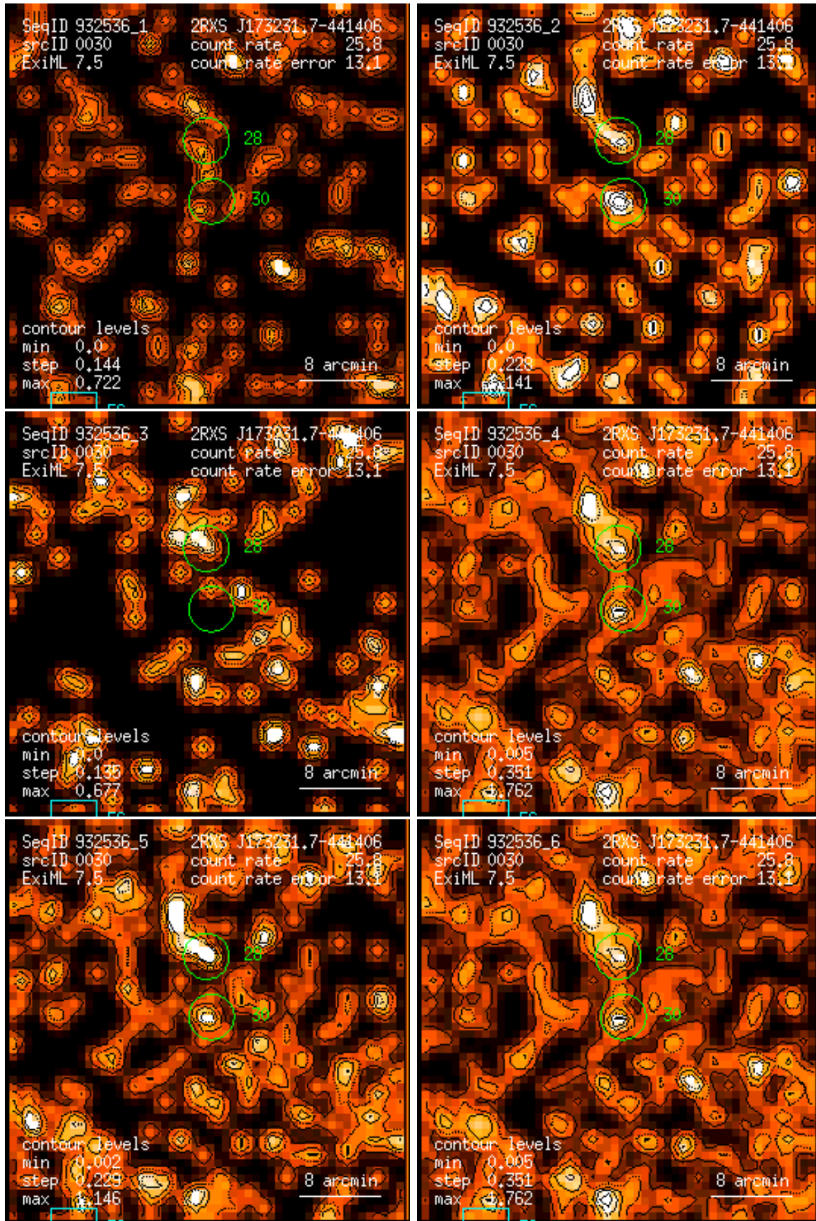
Figure 30: RASS 932536: detection 0030: band rate images, Gaussian filter: (1) PSPC channels 11 – 41, (2) 52 – 90, (3) 91 – 201, (4) 11 – 235, (5) 52 – 201, (6) 11 – 201. Broad band rates in counts/ks. Band rate contour levels in counts/ks/arcmin 2 .
