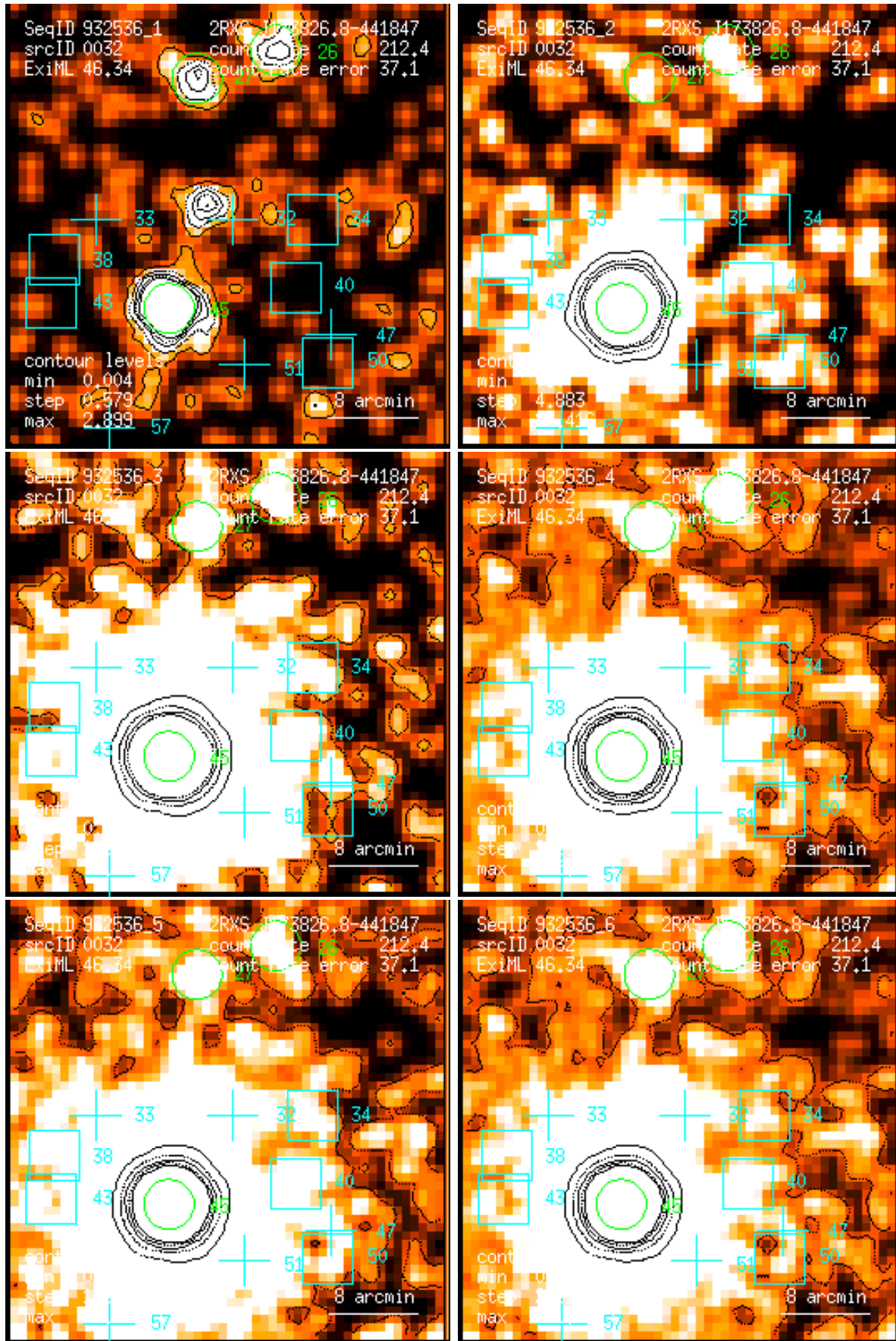
Figure 32: RASS 932536: detection 0032: band rate images, Gaussian filter: (1) PSPC channels 11 – 41, (2) 52 – 90, (3) 91 – 201, (4) 11 – 235, (5) 52 – 201, (6) 11 – 201. Broad band rates in counts/ks. Band rate contour levels in counts/ks/arcmin 2 .
