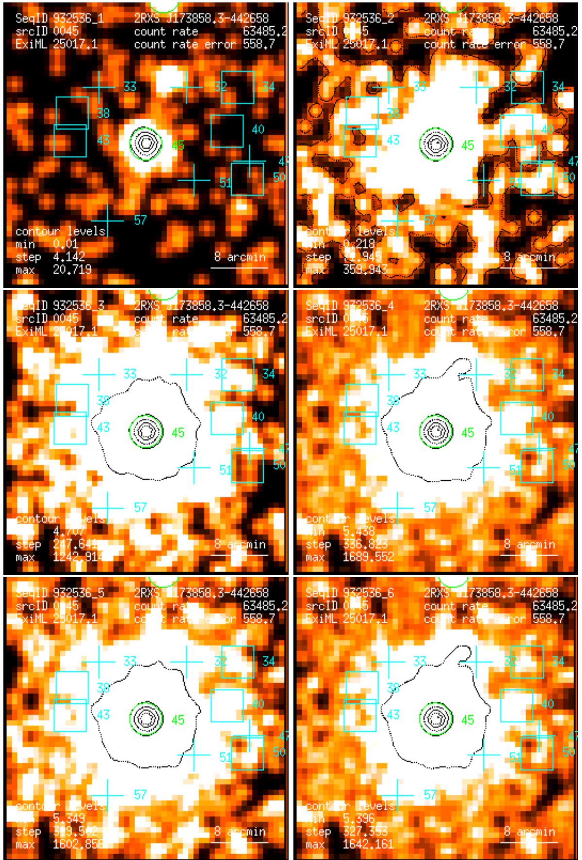
Figure 45: RASS 932536: detection 0045: band rate images, Gaussian filter: (1) PSPC channels 11 – 41, (2) 52 – 90, (3) 91 – 201, (4) 11 – 235, (5) 52 – 201, (6) 11 – 201. Broad band rates in counts/ks. Band rate contour levels in counts/ks/arcmin 2 .
