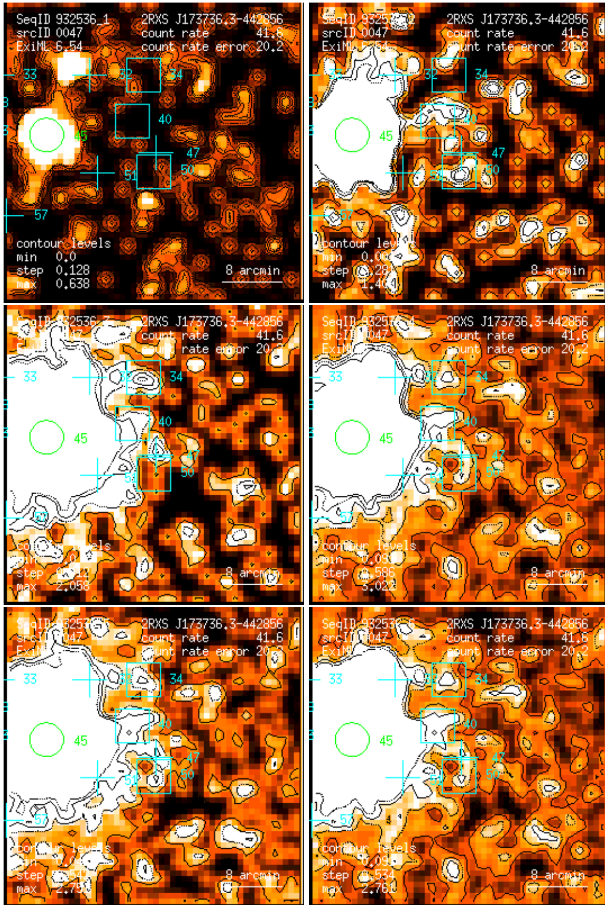
Figure 47: RASS 932536: detection 0047: band rate images, Gaussian filter: (1) PSPC channels 11 – 41, (2) 52 – 90, (3) 91 – 201, (4) 11 – 235, (5) 52 – 201, (6) 11 – 201. Broad band rates in counts/ks. Band rate contour levels in counts/ks/arcmin 2 .
