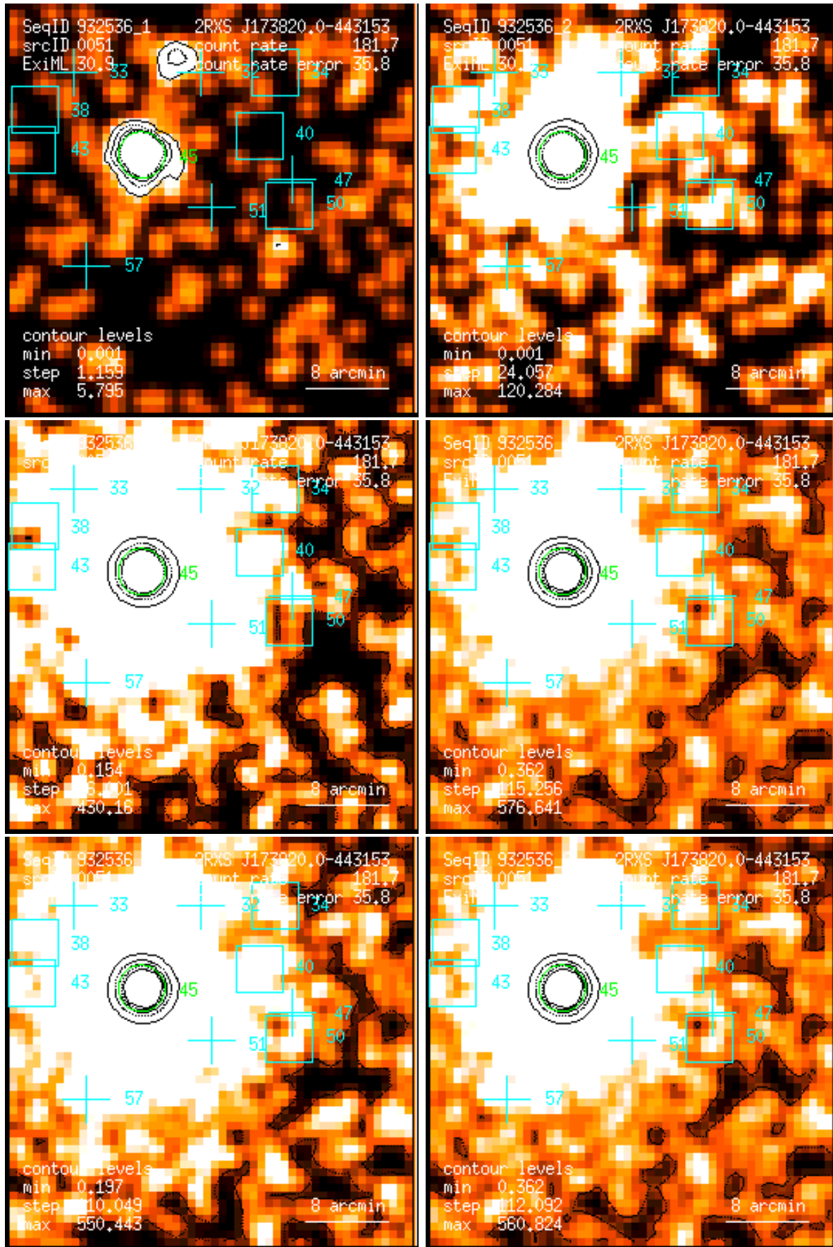
Figure 51: RASS 932536: detection 0051: band rate images, Gaussian filter: (1) PSPC channels 11 – 41, (2) 52 – 90, (3) 91 – 201, (4) 11 – 235, (5) 52 – 201, (6) 11 – 201. Broad band rates in counts/ks. Band rate contour levels in counts/ks/arcmin 2 .
