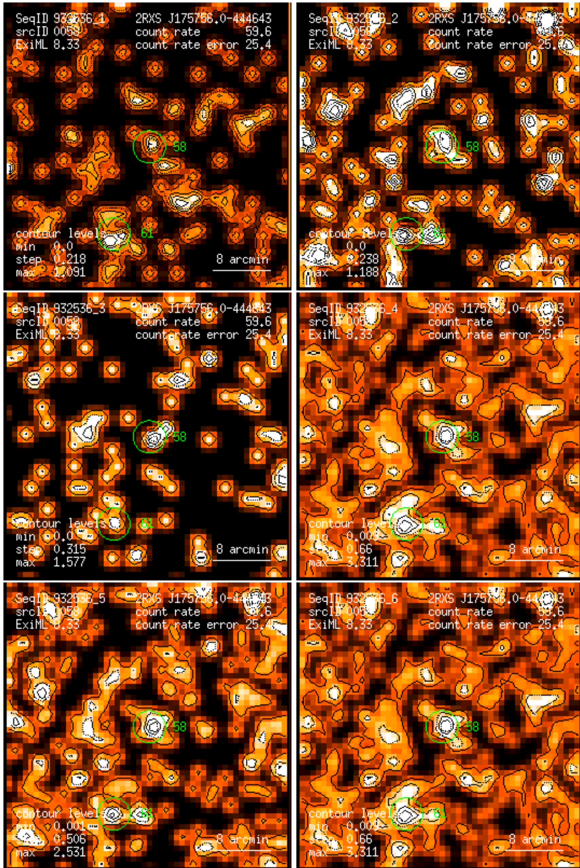
Figure 58: RASS 932536: detection 0058: band rate images, Gaussian filter: (1) PSPC channels 11 – 41, (2) 52 – 90, (3) 91 – 201, (4) 11 – 235, (5) 52 – 201, (6) 11 – 201. Broad band rates in counts/ks. Band rate contour levels in counts/ks/arcmin 2 .
