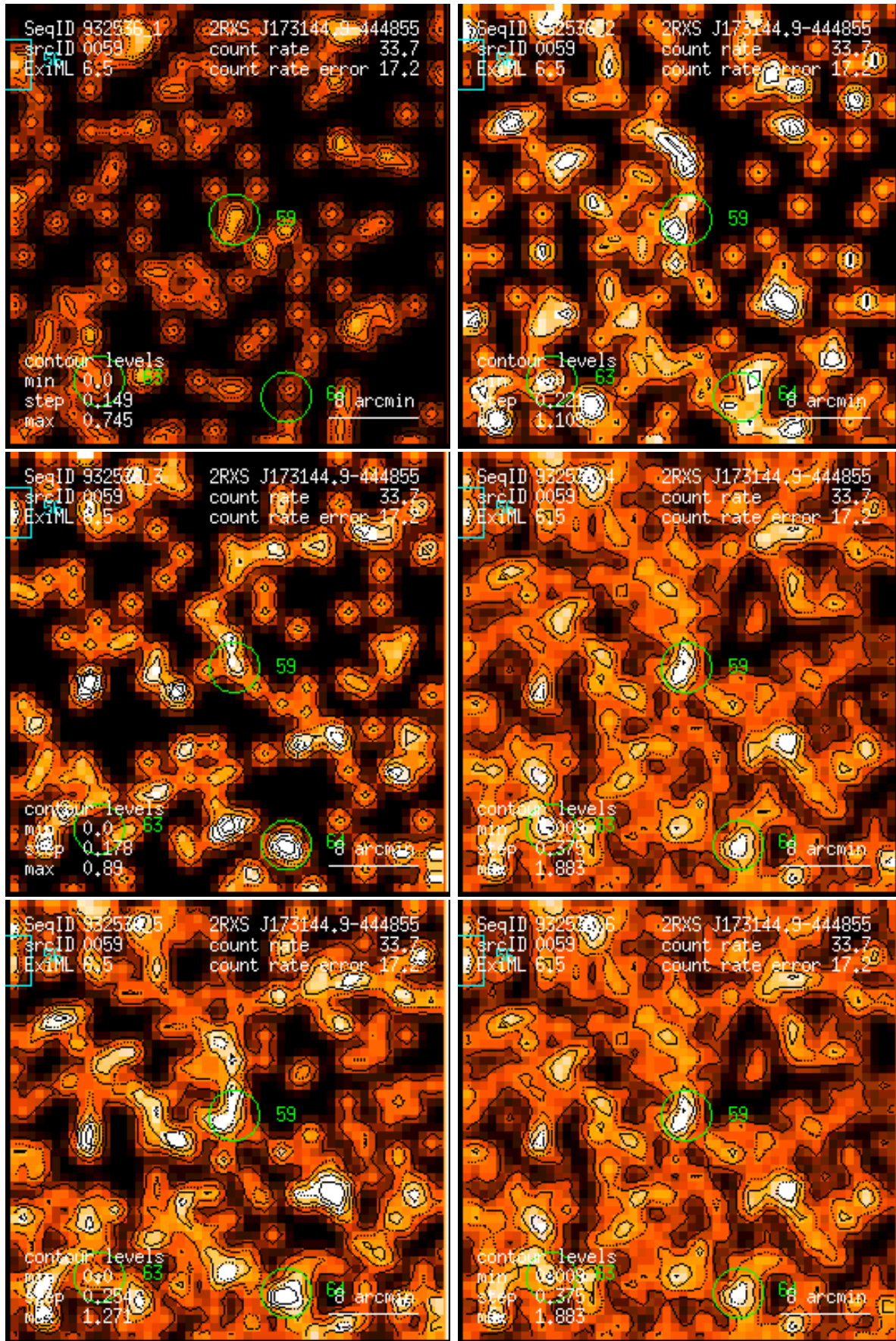
Figure 59: RASS 932536: detection 0059: band rate images, Gaussian filter: (1) PSPC channels 11 – 41, (2) 52 – 90, (3) 91 – 201, (4) 11 – 235, (5) 52 – 201, (6) 11 – 201. Broad band rates in counts/ks. Band rate contour levels in counts/ks/arcmin 2 .
