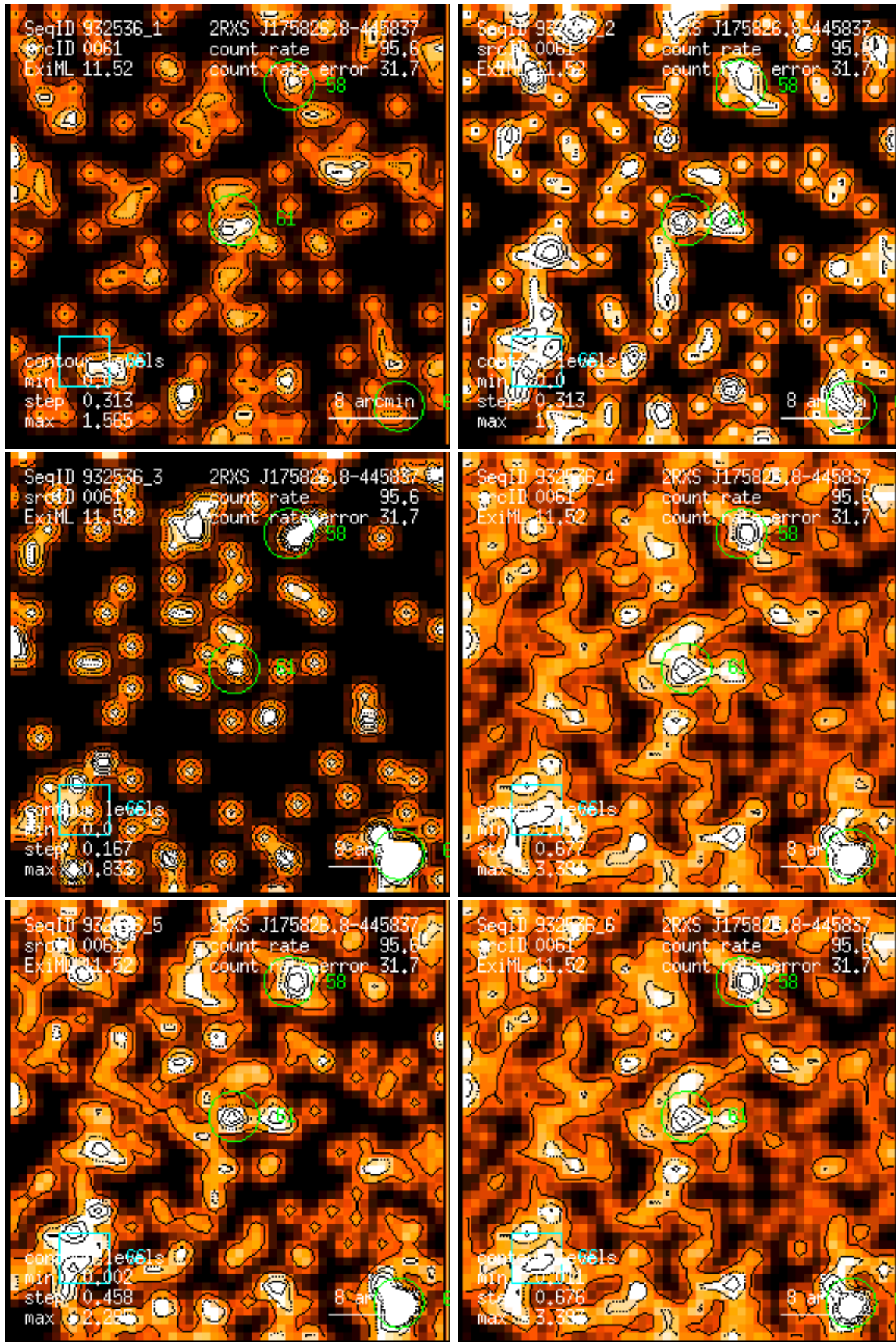
Figure 61: RASS 932536: detection 0061: band rate images, Gaussian filter: (1) PSPC channels 11 – 41, (2) 52 – 90, (3) 91 – 201, (4) 11 – 235, (5) 52 – 201, (6) 11 – 201. Broad band rates in counts/ks. Band rate contour levels in counts/ks/arcmin 2 .
