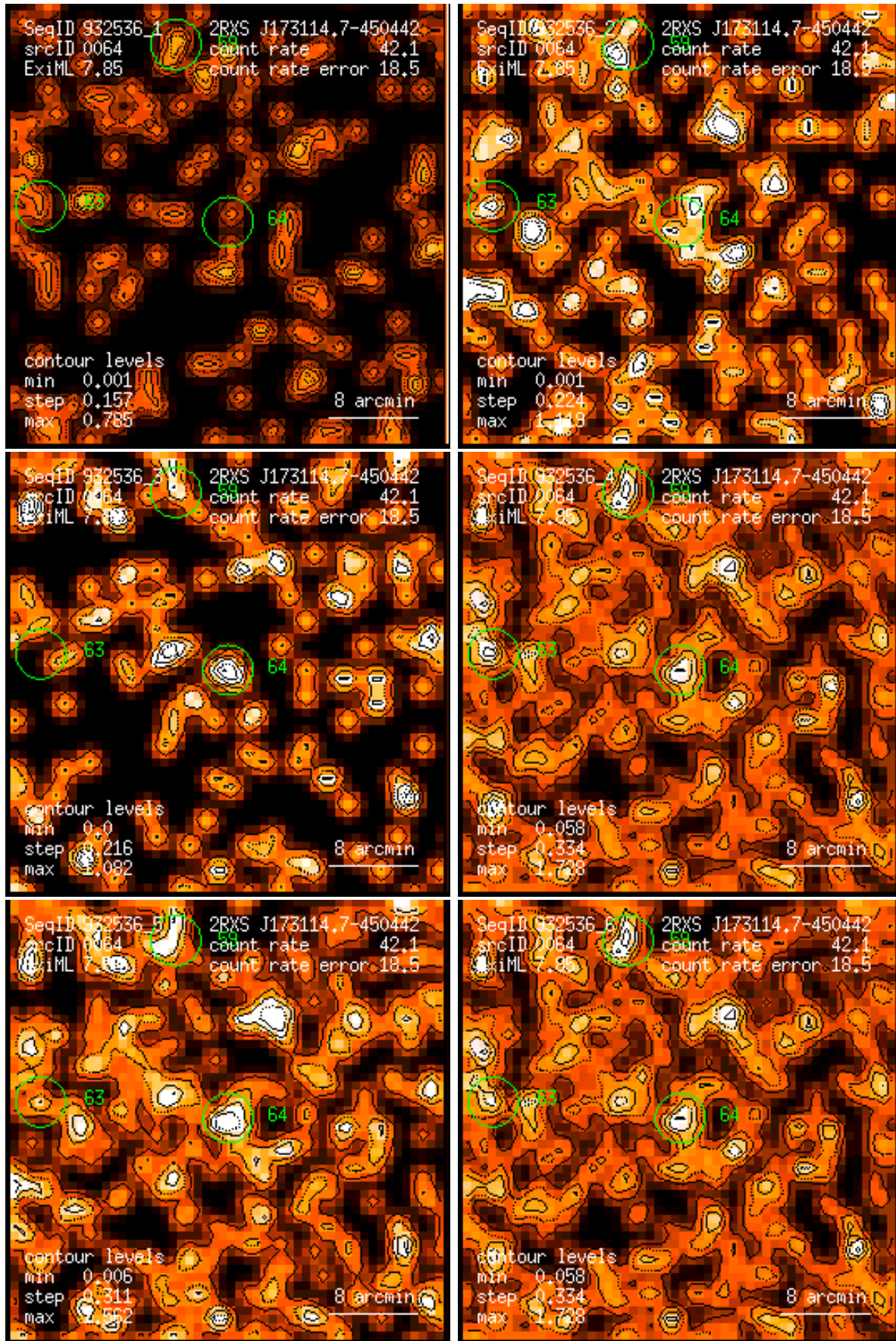
Figure 64: RASS 932536: detection 0064: band rate images, Gaussian filter: (1) PSPC channels 11 – 41, (2) 52 – 90, (3) 91 – 201, (4) 11 – 235, (5) 52 – 201, (6) 11 – 201. Broad band rates in counts/ks. Band rate contour levels in counts/ks/arcmin 2 .
