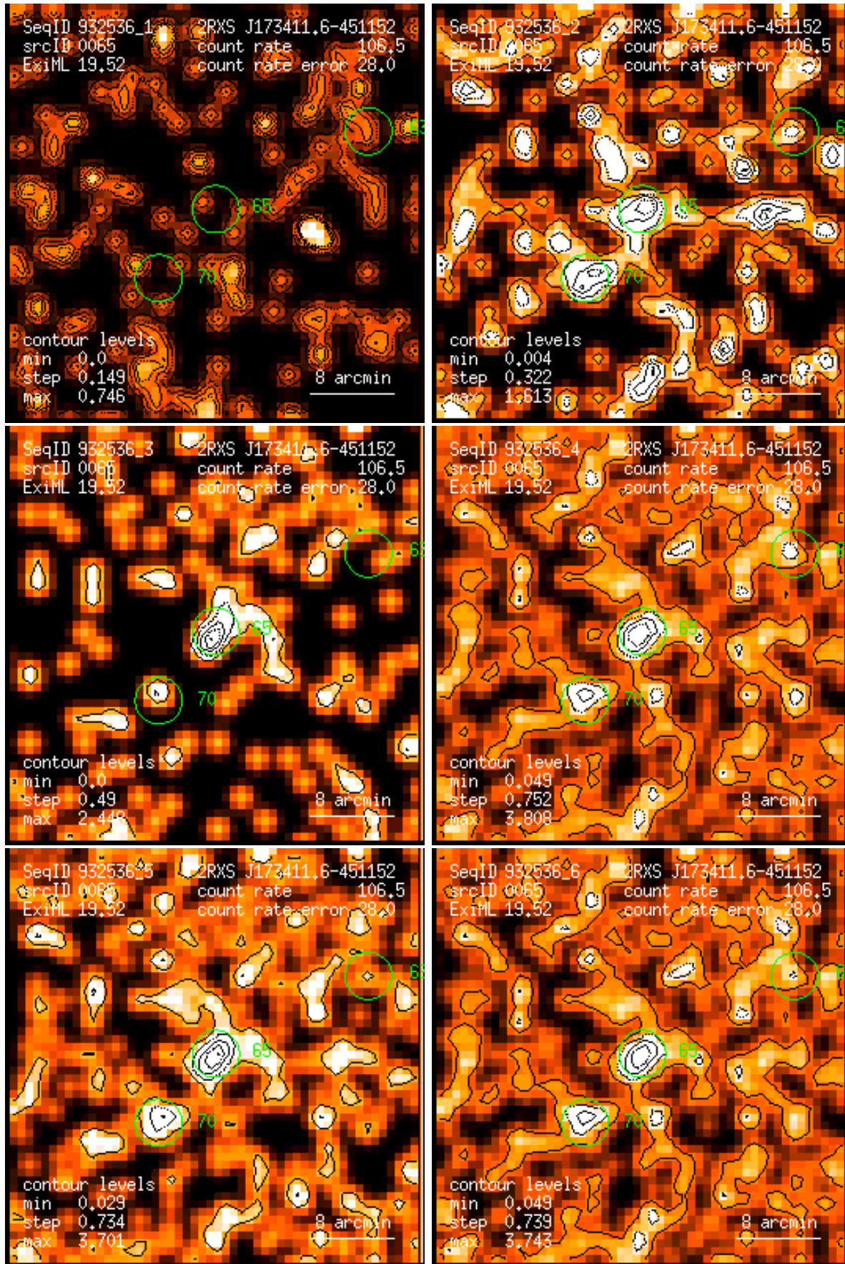
Figure 65: RASS 932536: detection 0065: band rate images, Gaussian filter: (1) PSPC channels 11 – 41, (2) 52 – 90, (3) 91 – 201, (4) 11 – 235, (5) 52 – 201, (6) 11 – 201. Broad band rates in counts/ks. Band rate contour levels in counts/ks/arcmin 2 .
