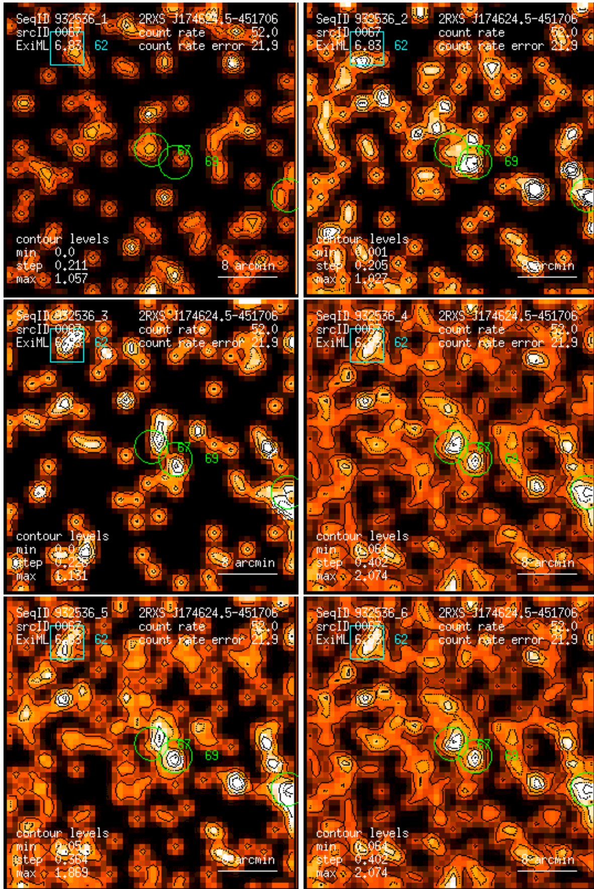
Figure 67: RASS 932536: detection 0067: band rate images, Gaussian filter: (1) PSPC channels 11 – 41, (2) 52 – 90, (3) 91 – 201, (4) 11 – 235, (5) 52 – 201, (6) 11 – 201. Broad band rates in counts/ks. Band rate contour levels in counts/ks/arcmin 2 .
