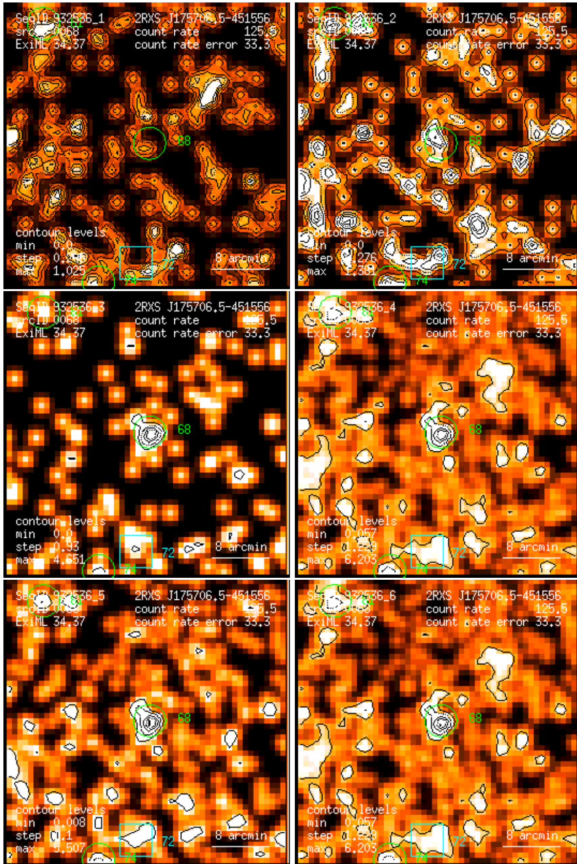
Figure 68: RASS 932536: detection 0068: band rate images, Gaussian filter: (1) PSPC channels 11 – 41, (2) 52 – 90, (3) 91 – 201, (4) 11 – 235, (5) 52 – 201, (6) 11 – 201. Broad band rates in counts/ks. Band rate contour levels in counts/ks/arcmin 2 .
