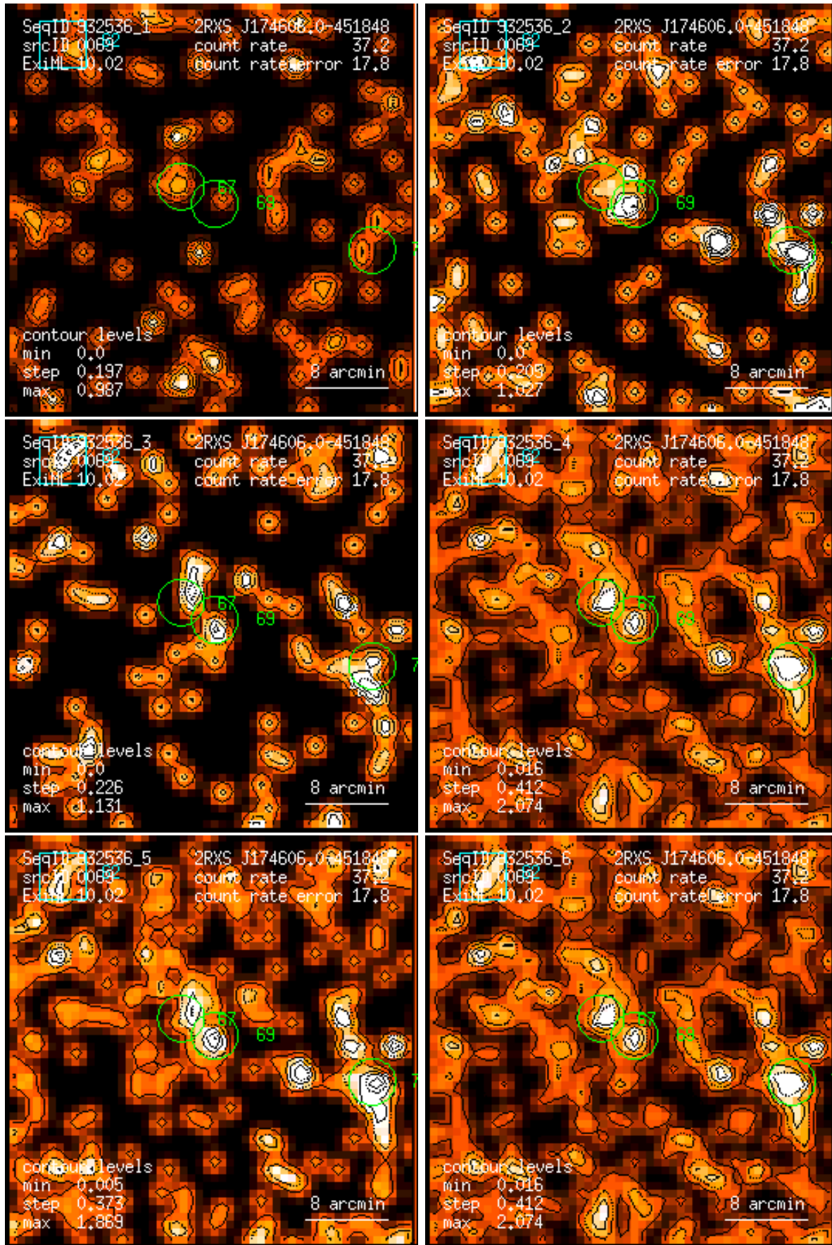
Figure 69: RASS 932536: detection 0069: band rate images, Gaussian filter: (1) PSPC channels 11 – 41, (2) 52 – 90, (3) 91 – 201, (4) 11 – 235, (5) 52 – 201, (6) 11 – 201. Broad band rates in counts/ks. Band rate contour levels in counts/ks/arcmin 2 .
