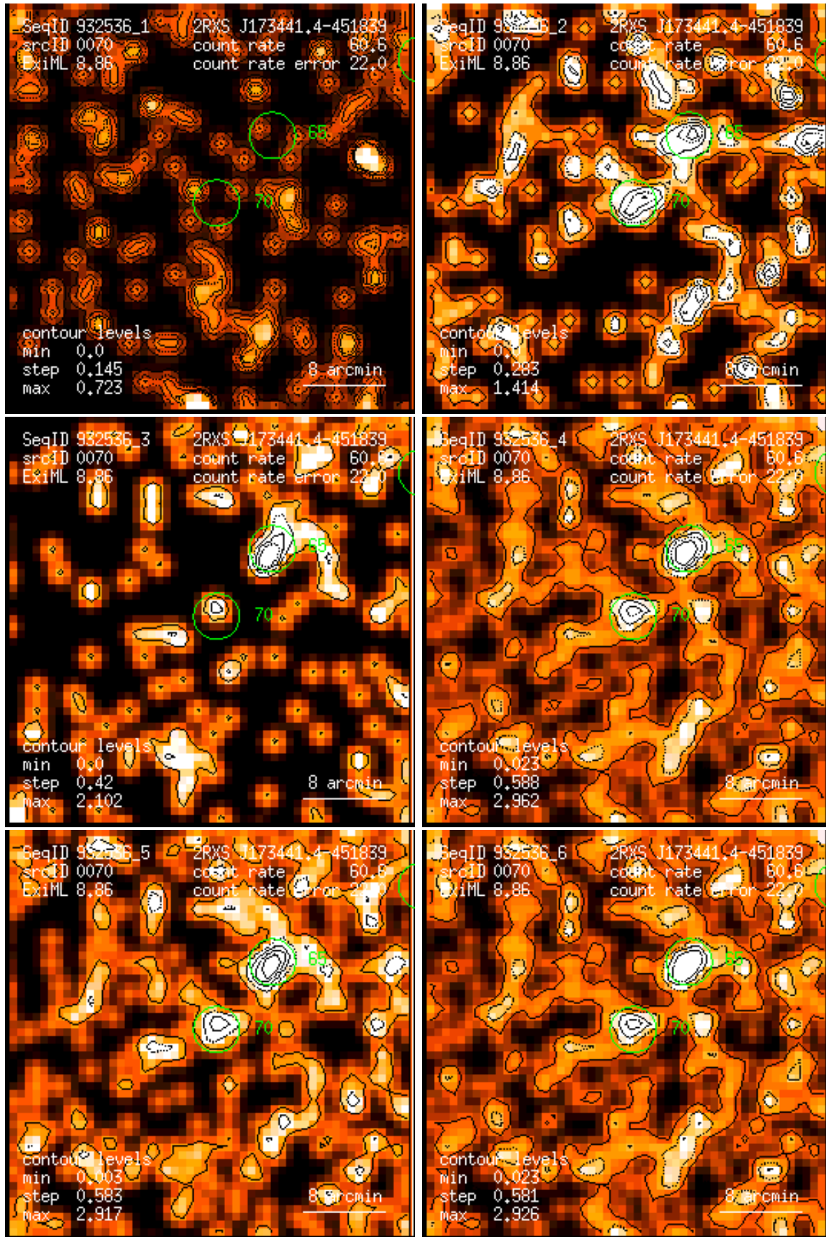
Figure 70: RASS 932536: detection 0070: band rate images, Gaussian filter: (1) PSPC channels 11 – 41, (2) 52 – 90, (3) 91 – 201, (4) 11 – 235, (5) 52 – 201, (6) 11 – 201. Broad band rates in counts/ks. Band rate contour levels in counts/ks/arcmin 2 .
